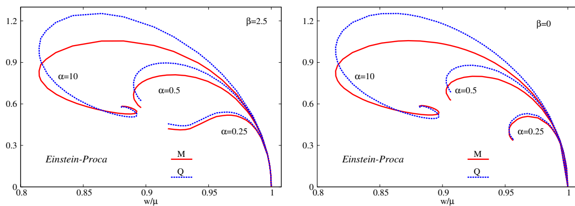
Figure 6. Same as Figure 4 for Proca stars.
