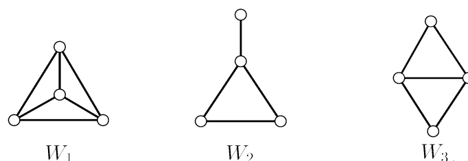
Figure 1. Three graphs W_1 , W_2 and W_3 of order 4.
