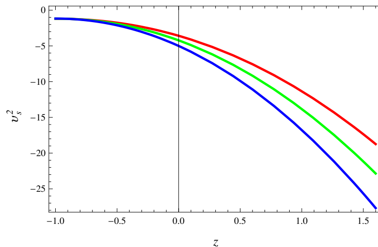
Figure 5. Plot of v_s^2 against z for conserved EMT for m_1 = 1.7 (red), m_2 = 1.8 (green) and m_3 = 1.9 (blue) illustrates instability of the model.
