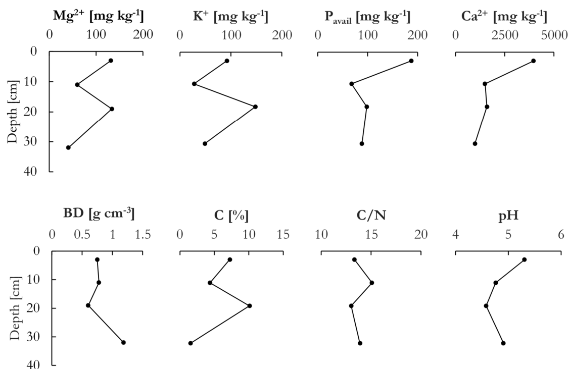
Figure 3. Selected chemical and physical properties of the soil profile. P_{\text{avail}} : plant-available P; BD: bulk density.
