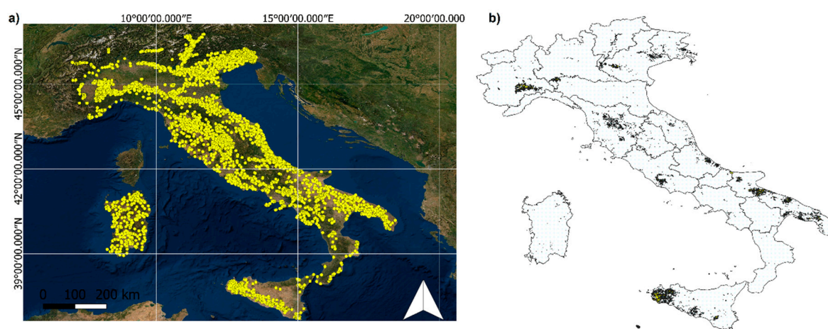
Figure 1. (a) Identification of the centroids of the 3686 sample vineyards (yellow dots). (b) Political map of Italy with the vineyard land cover (shading). Source: Copernicus CORINE Land Cover (CLC) 2018 ( https://land.copernicus.eu/ ).
