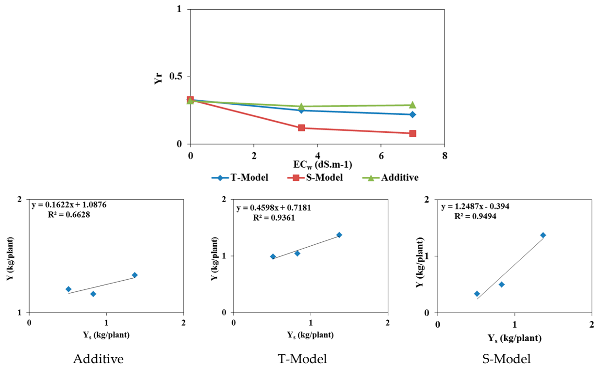
Figure 11. The effect of saline irrigation water on tomatoes' relative yield ( Y_r ) [—] ( top ) and the relationships between the actual ( Y ) and simulated ( Y_s ) yields (kg/plant) ( bottom ) using the three stress response models (Additive, T-Model, and S-Model) incorporated in Hydrus-1D (pot experiments).
