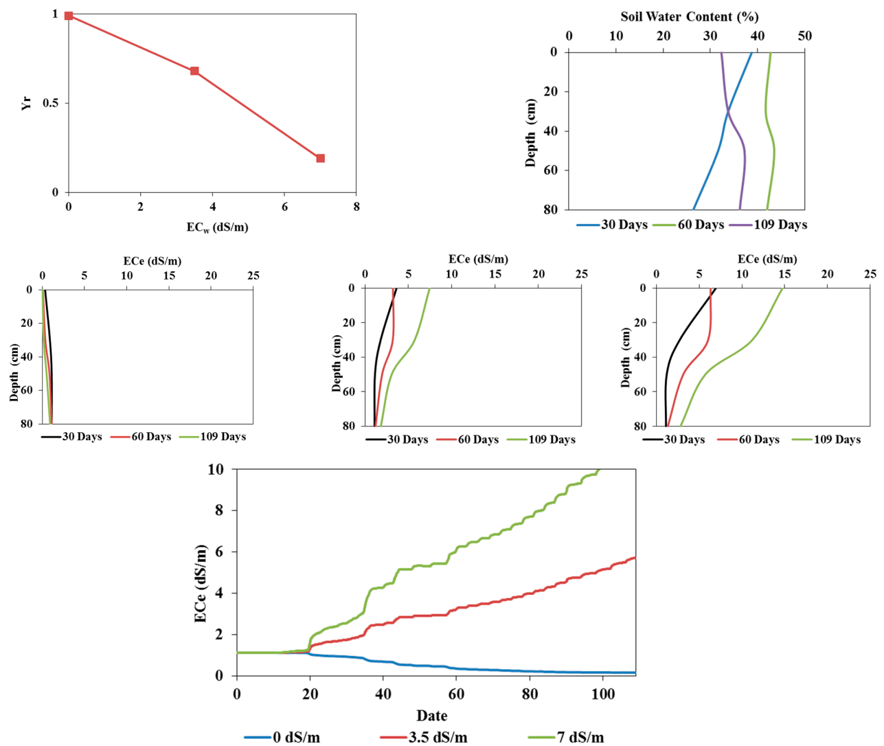
Figure 12. Effects of a temperature increase of 2 °C on tomatoes cultivated in field conditions: relative yield as a function of irrigation water salinity ( top left ); soil water content profiles at 30, 60, and 109 days when irrigated with freshwater ( top right ); soil salinity profiles at 30, 60, and 109 days ( middle row ) when irrigated with fresh water ( left ) and saline waters of 3.5 ( middle ) and 7 ( right ) dS/m; and average root zone salinity when irrigated with fresh water and saline waters of 3.5 and 7 dS/m ( bottom ).
