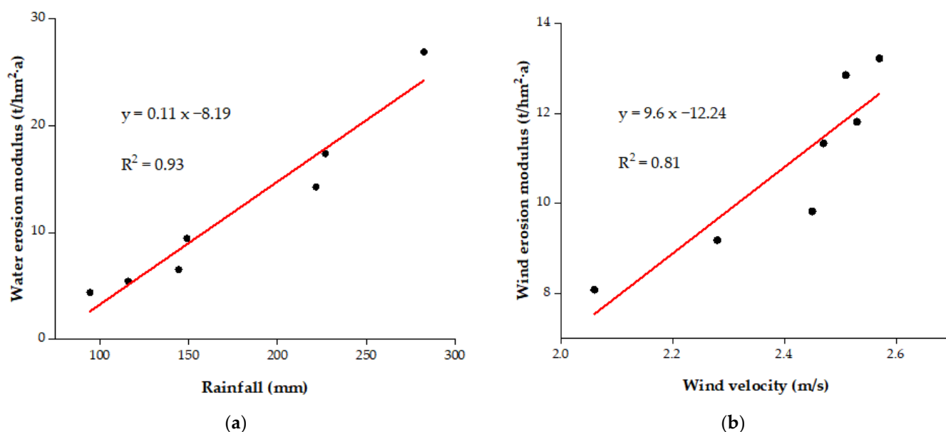
Figure 7. Relationship between soil erosion and meteorological factors in Baotou City. (a) Relationship between water erosion modulus and precipitation; (b) relationship between wind erosion modulus and wind velocity.
