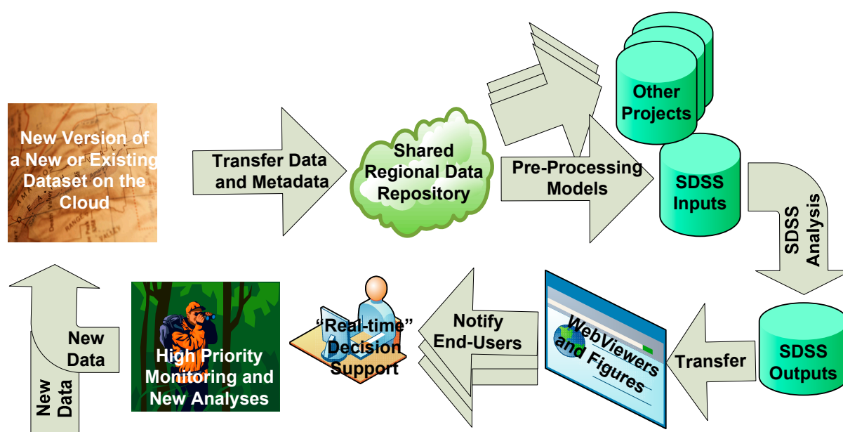
Figure 3. Simplified workflow of a “living” SDSS (spatial decision support system), which is able to provide updated products as conditions change. A challenge in a “living” SDSS is to automate, as much as practical, all the steps within each arrow, and eventually, the linking of all the arrows.
