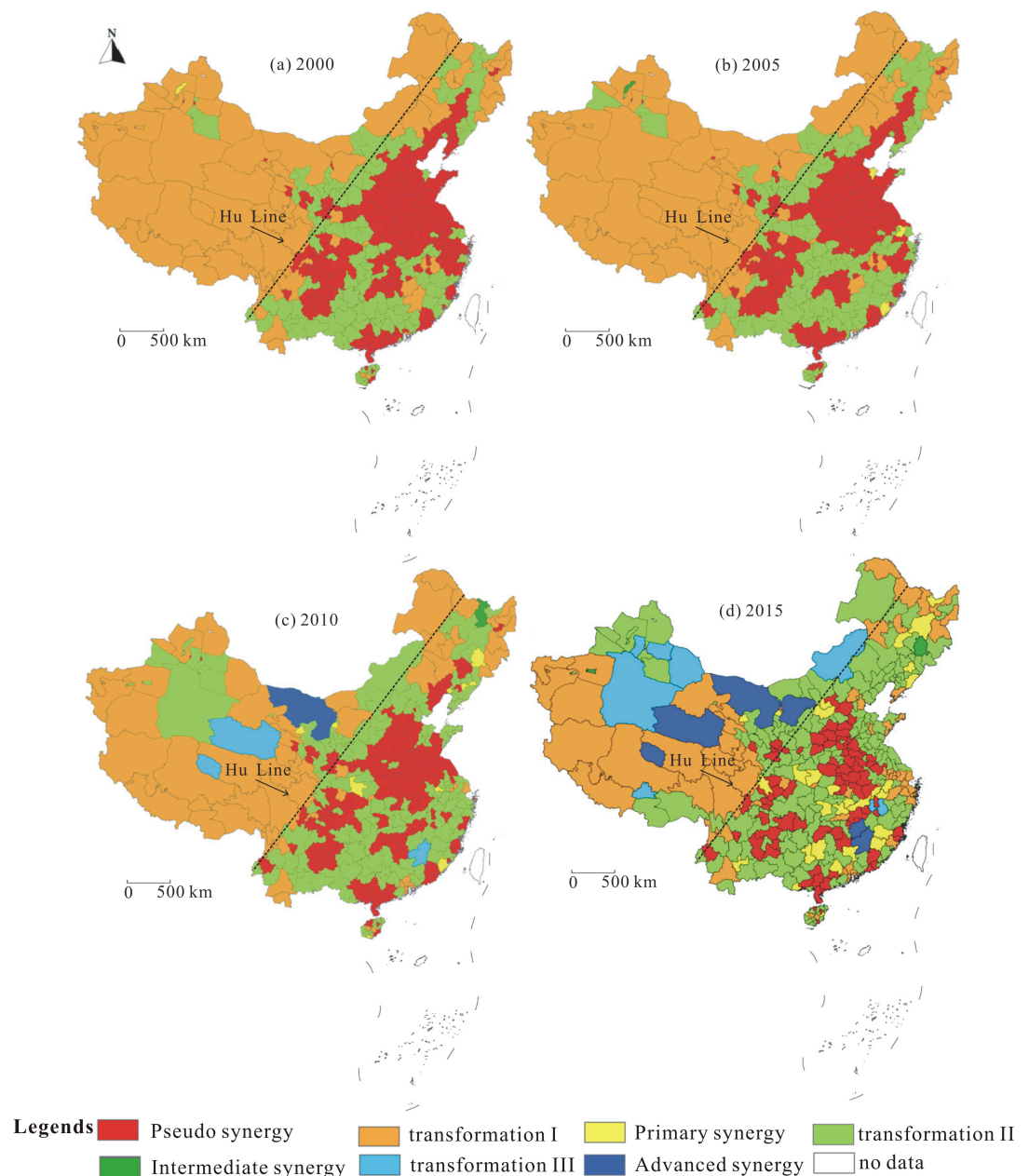
Figure 2. Spatial distribution characteristics of the GEP–GDP synergy in the Chinese mainland during the investigation period.
