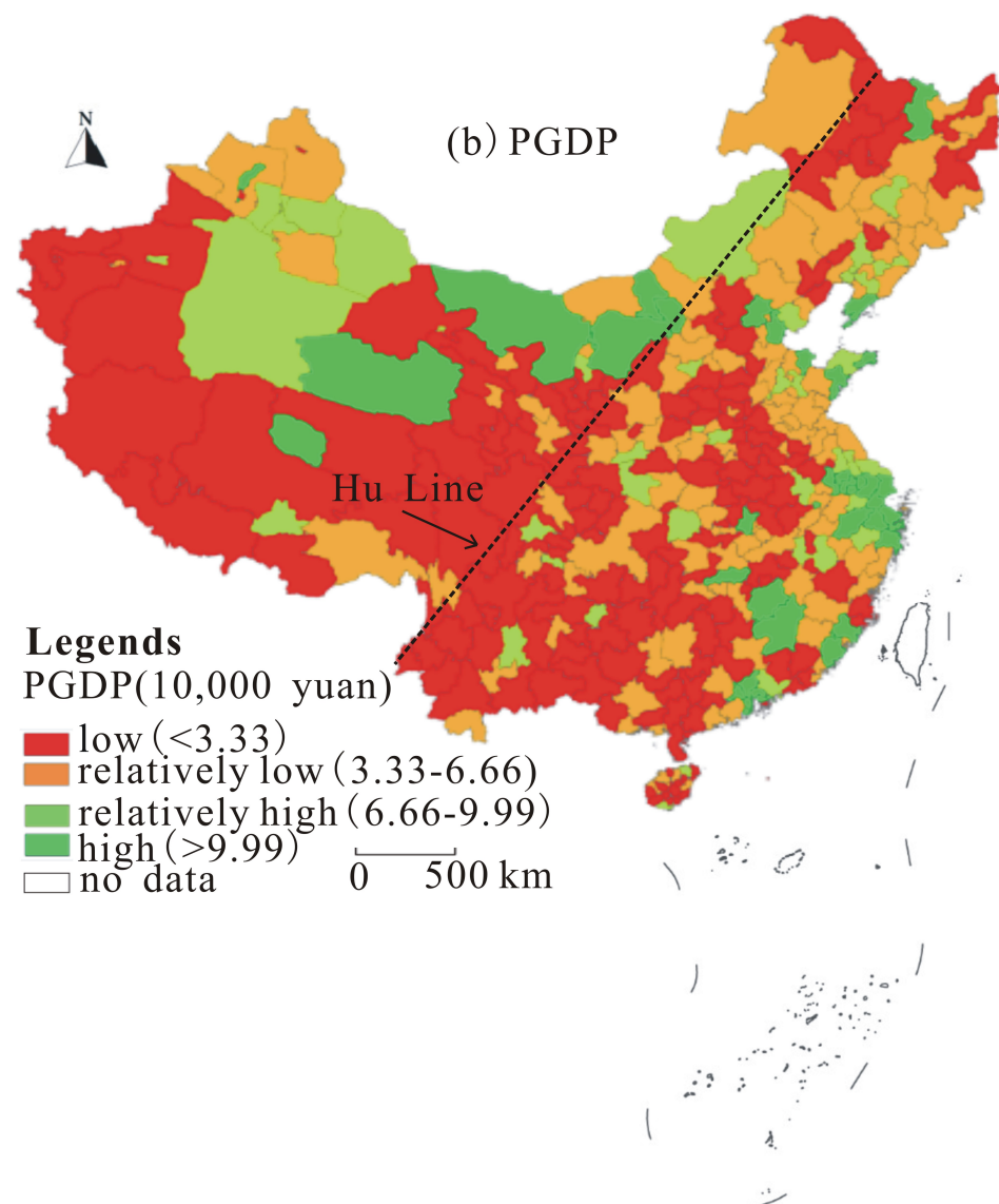
Figure 1. Spatial distribution characteristics of the PGEP and PGDP in the Chinese mainland.
