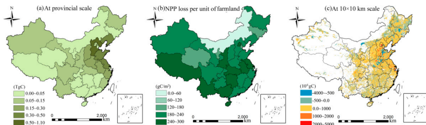
Figure 6. Spatial distribution of the loss of farmland NPP due to rural settlement expansion from 2000 to 2020.
