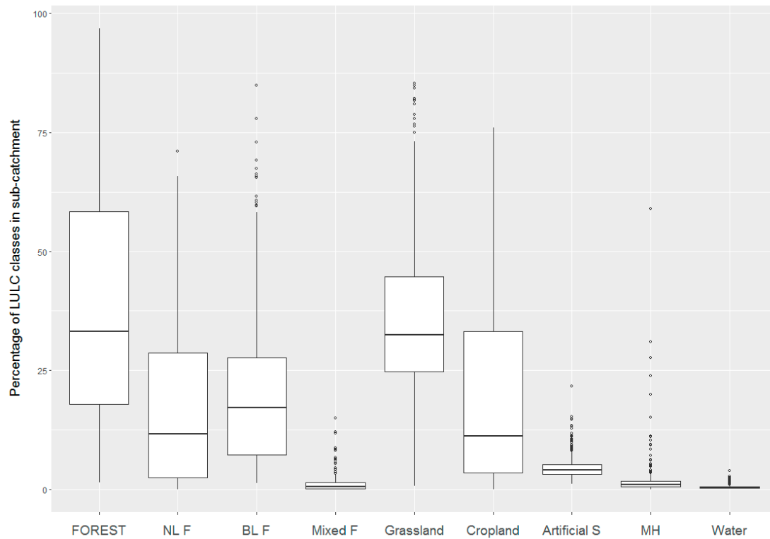
Figure S1. LULC percentages in the sub-catchments with NL F needle-leaved forest, BL F: broad-leaved forest, S: Surfaces and MH: shrubs–heathlands and moorlands.
