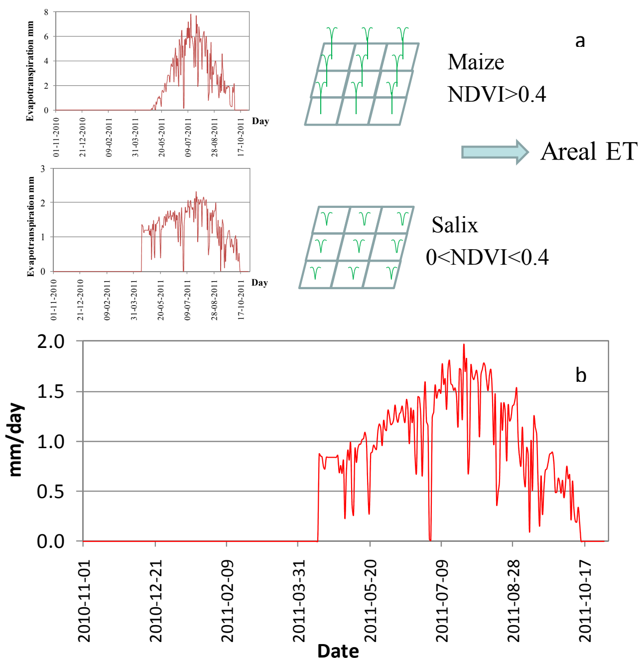
Figure 4. Up-scaling approach for areal evapotranspiration with sap flow measurements and NDVI values (a); and the estimated areal evapotranspiration (b).
