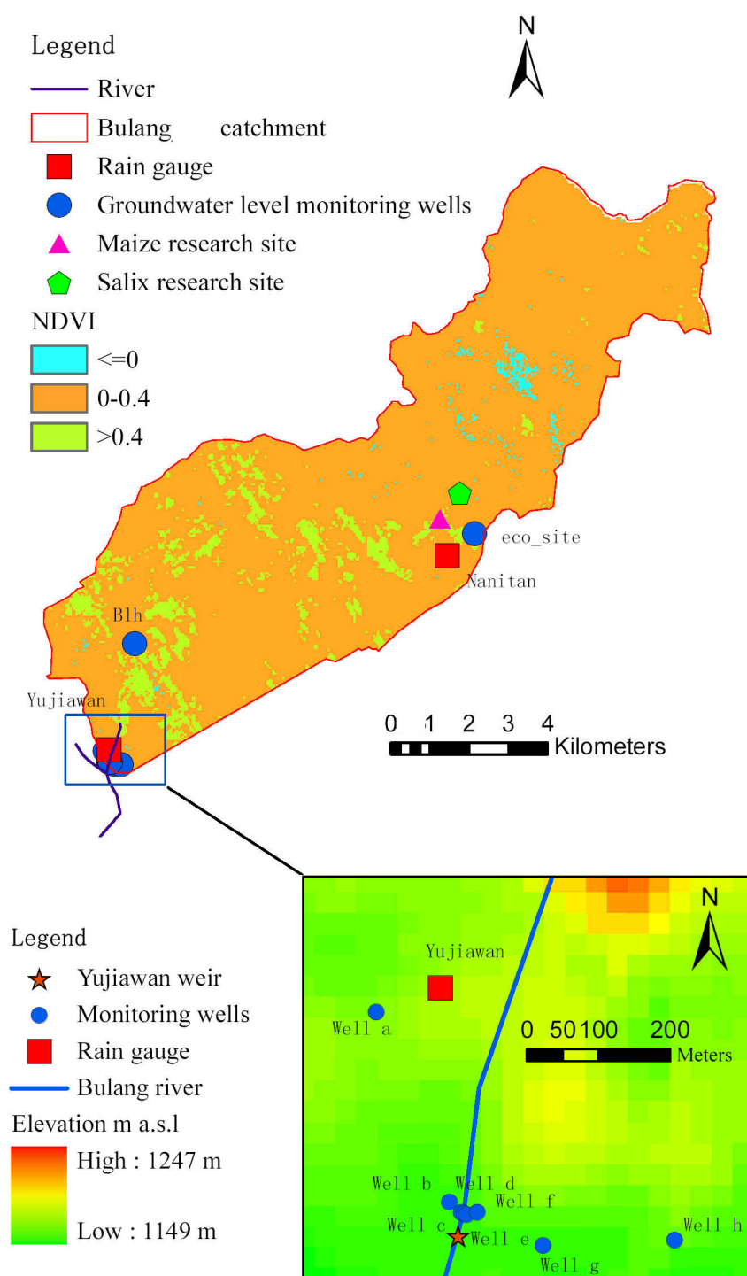
Figure 2. NDVI map of the Bulang catchment, interpretation of remote sensing data from (TM) image, observed on August 2011.
