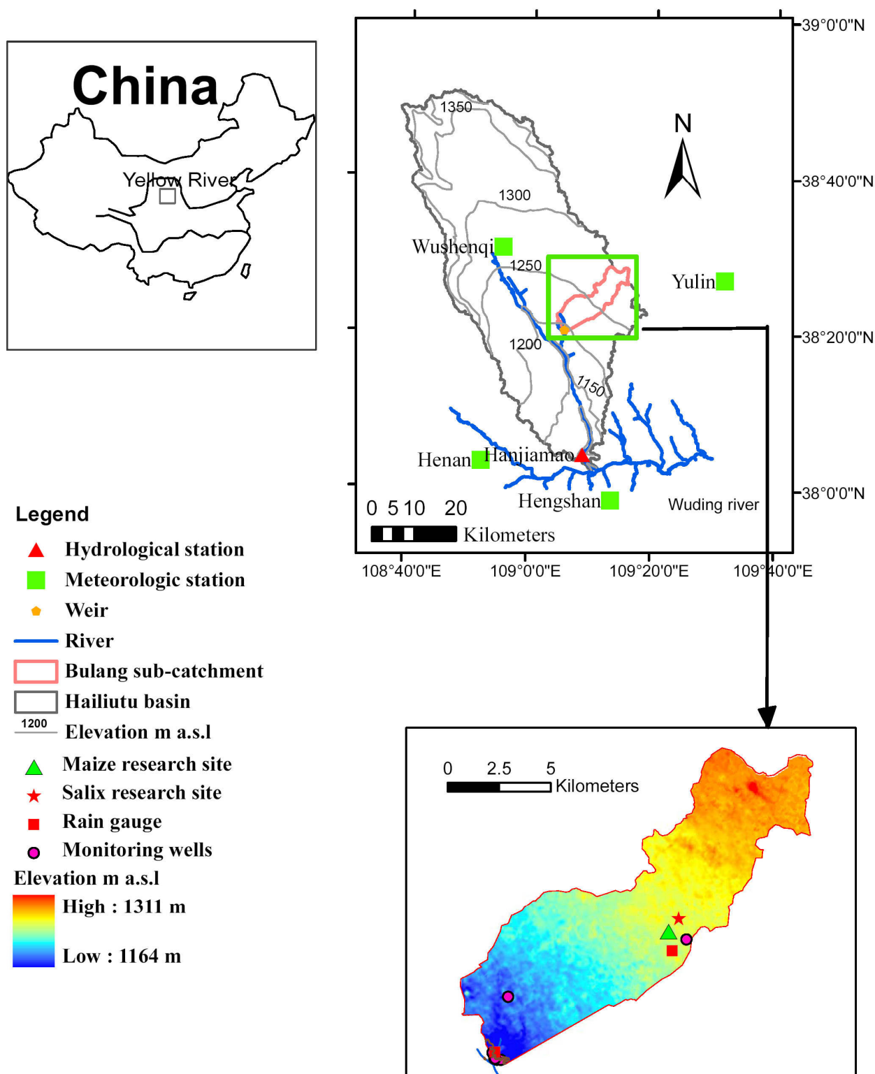
Figure 1. Location of the Bulang sub-catchment within the Hailutu basin in Northwest China, the location of sap flow measurements for maize and salix, hydrological and meteorological stations, groundwater level monitoring wells, and the digital elevation model.
