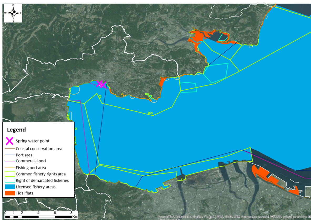
Figure A1. Beppu Bay—Multiple overlay map. Source: [48].
