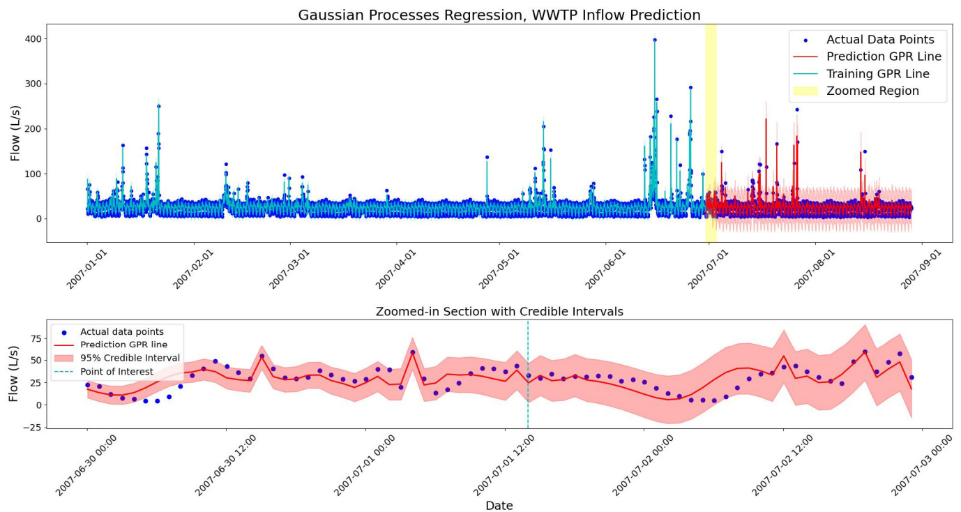
Figure 4. Gaussian process regression model on 6 months of training and 2 months of test data ( top ). The regression lines are shown in blue and red for training and test sets, respectively. The first 3 days of the test set is selected for a detailed illustration ( bottom ).
