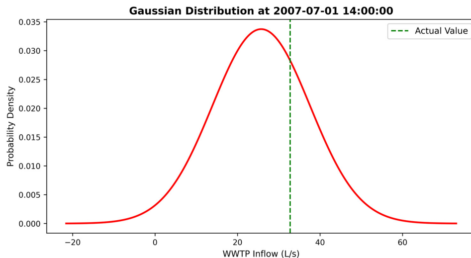
Figure 5. Gaussian distribution of the predicted WWTP inflow at 2007-07-01 at 14:00 p.m. The green dashed line shows the actual test point value. The distribution's domain is selected as \pm 4 standard deviation of the distribution for a better illustration.
