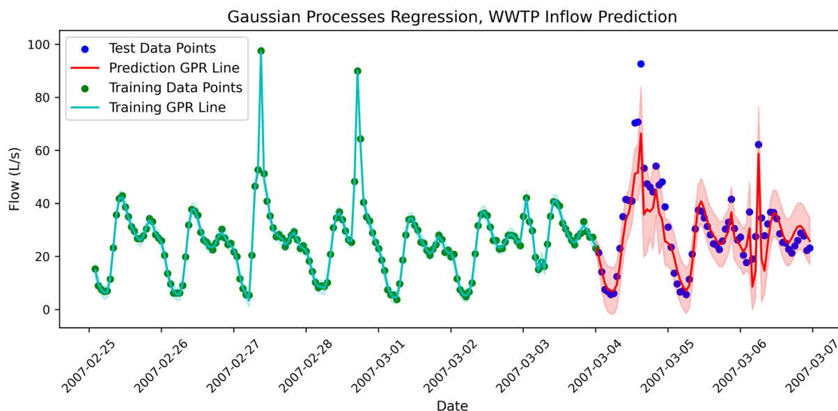
Figure 10. WWTP inflow prediction with seven days of training data using Gaussian process regression. The test period is three days, and the 95% credible interval is used to show the uncertainty around the predictions.
