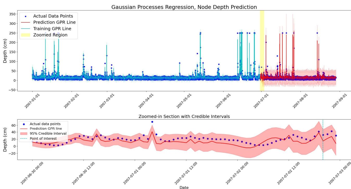
Figure 6. Water depth forecasting at node J15 for 2 months ( top ). GPR line at training and test datasets are illustrated in blue and red, respectively. The first 3 days of the test set is selected for a detailed illustration ( bottom ).
