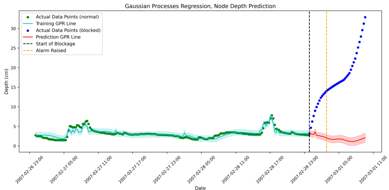
Figure 9. Blockage detection by water depth forecasting at J2 node. The prediction for 10 h has been presented by red line and the observed values have been presented by blue bullets. After three hours of consequent data points falling outside the bounds, an alarm is raised showing a probable blockage. The time interval between points is 15 min.
