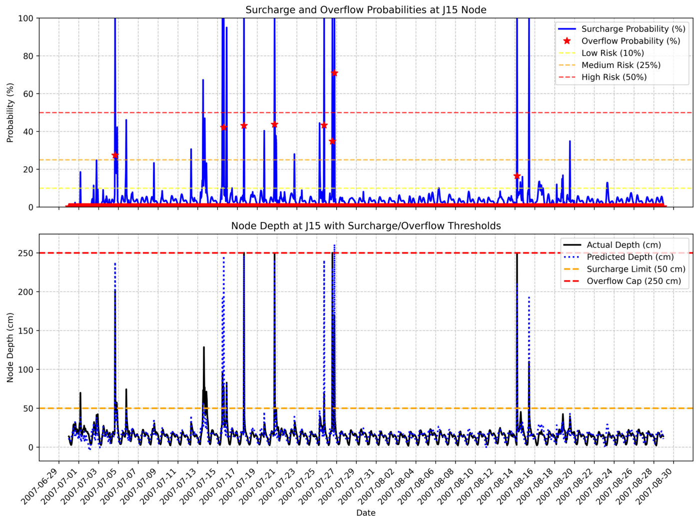
Figure 8. (Top): the probability of surcharge and overflow in the selected manhole. Blue line shows the probability of surcharge over time, and the red stars show the probability of an overflow from the manhole in each timestep. The dashed lines are drawn to divide the space into low, medium and high-risk zones. (Bottom): actual and predicted water depth at the selected manhole. Surcharge and overflow limits are shown with dashed lines.
