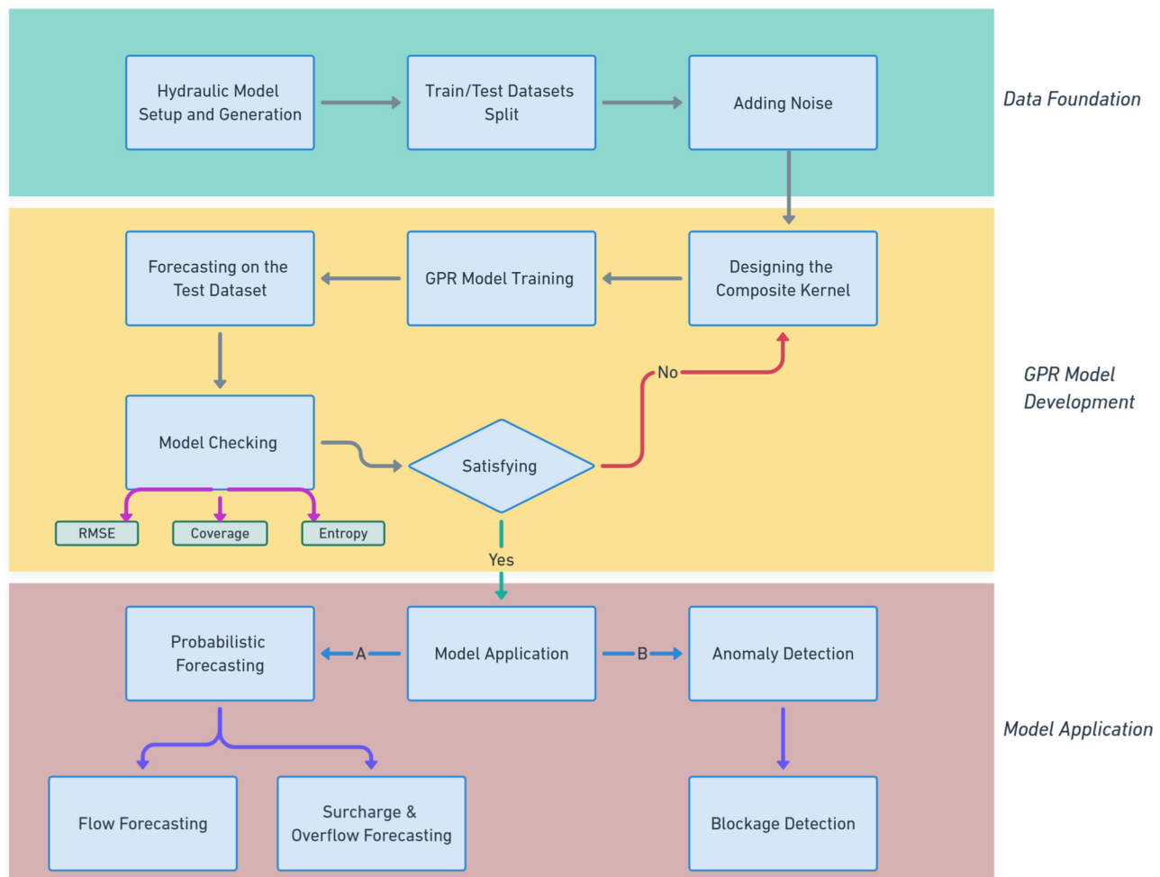
Figure 2. Flowchart of the research methodology, illustrating the stages from data foundation to the final applications. This process starts from preparing training and test datasets and then makes the composite kernel for the GPR model development. Finally, the built model comes to different applications.
