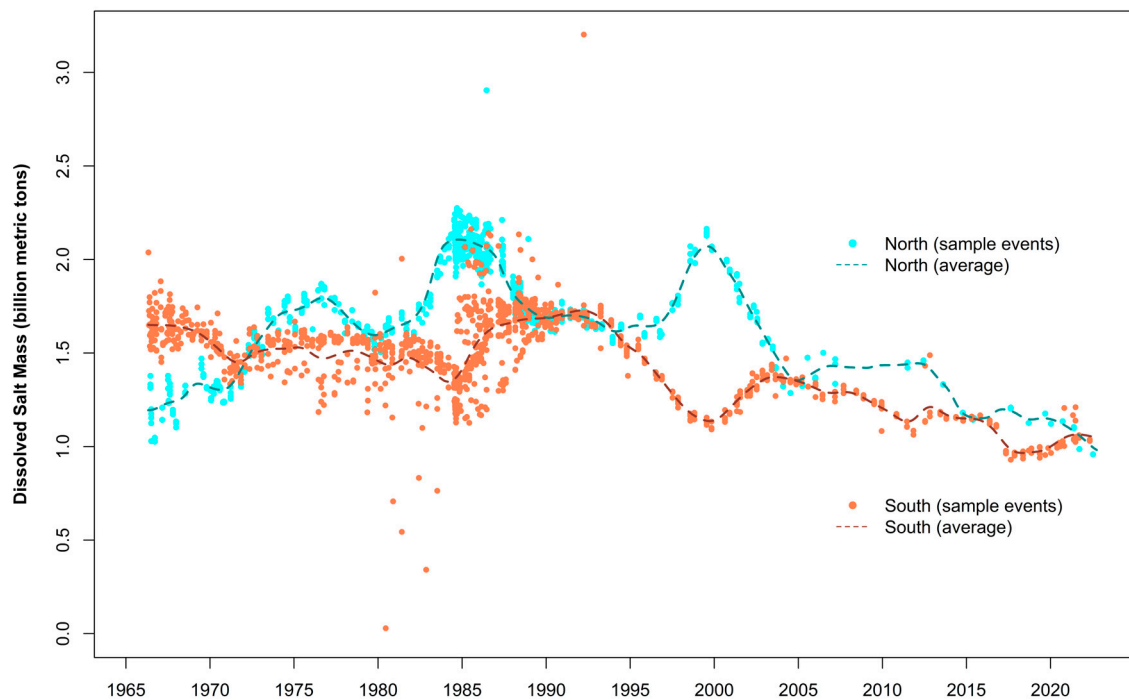
Figure 7. North and south arm average dissolved salt mass over the period of record at GSL measurement sites (Figure 1). Point values were calculated using all measurements at a single site on a given date. Dashed lines represent the estimated monthly time series.
