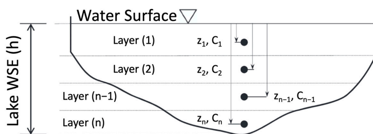
Figure 4. Hypothetical lake at WSE h with n number of measurements at depth on a given day. Cross-sections indicate layers used to calculate average dissolved salt mass and average salinity. Adapted with permission from Ref. [26], Copyright American Geophysical Union, 2012.
