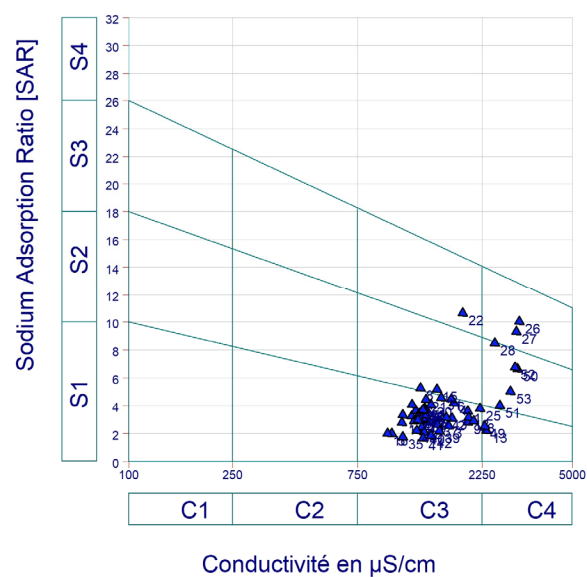
Figure 9. USSS diagram for irrigation purposes.
