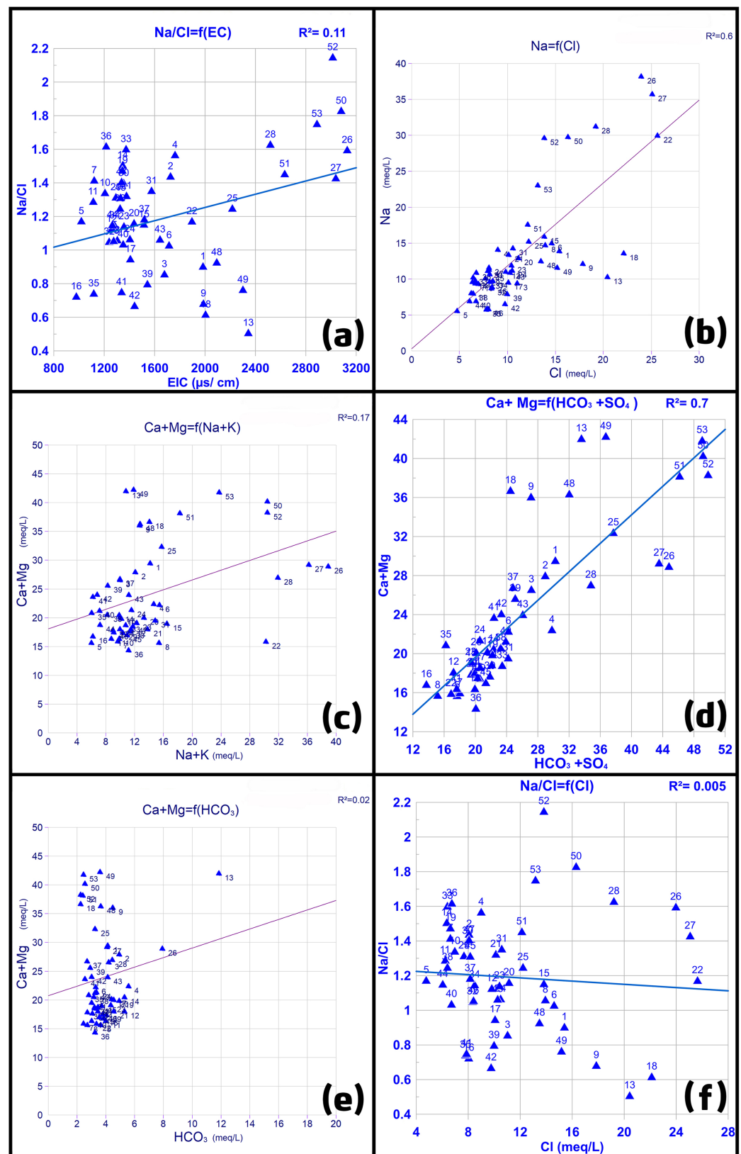
Figure 7. Correlations and ratios among different major ions: (a) \text{Na/Cl} and \text{EIC} ; (b) \text{Na} and \text{Cl} ; (c) \text{Ca} + \text{Mg} and \text{Na} + \text{K} ; (d) \text{Ca} + \text{Mg} and \text{SO}_4 + \text{HCO}_3 ; (e) \text{Ca} + \text{Mg} and \text{HCO}_3 ; (f) \text{Na/Cl} and \text{Cl} .
