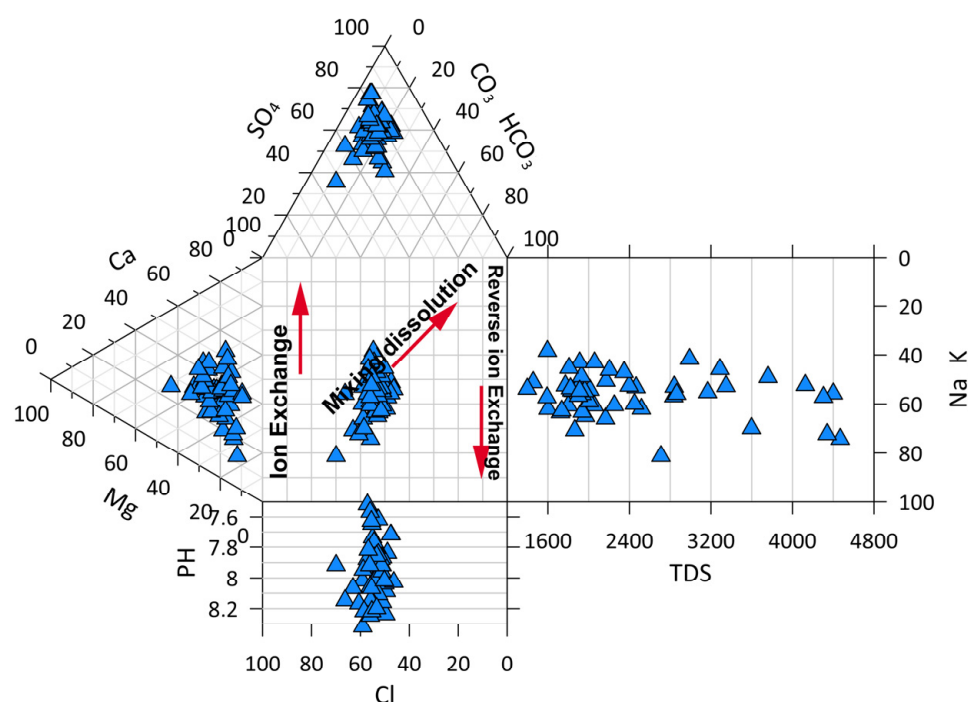
Figure 6. Durov diagram showing the key mechanisms controlling groundwater geochemistry.
