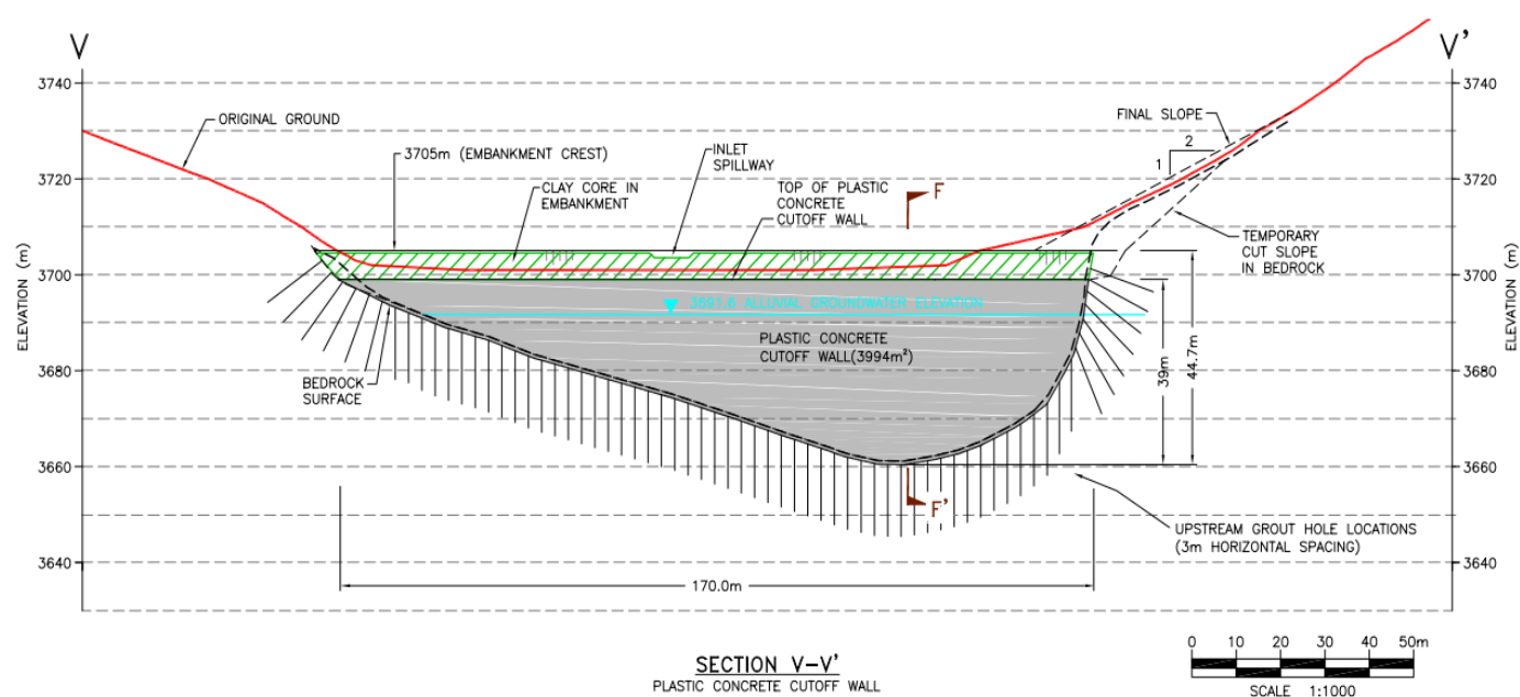
Figure 8. Example of plastic concrete slurry wall–grout curtain system in TSF dam.
