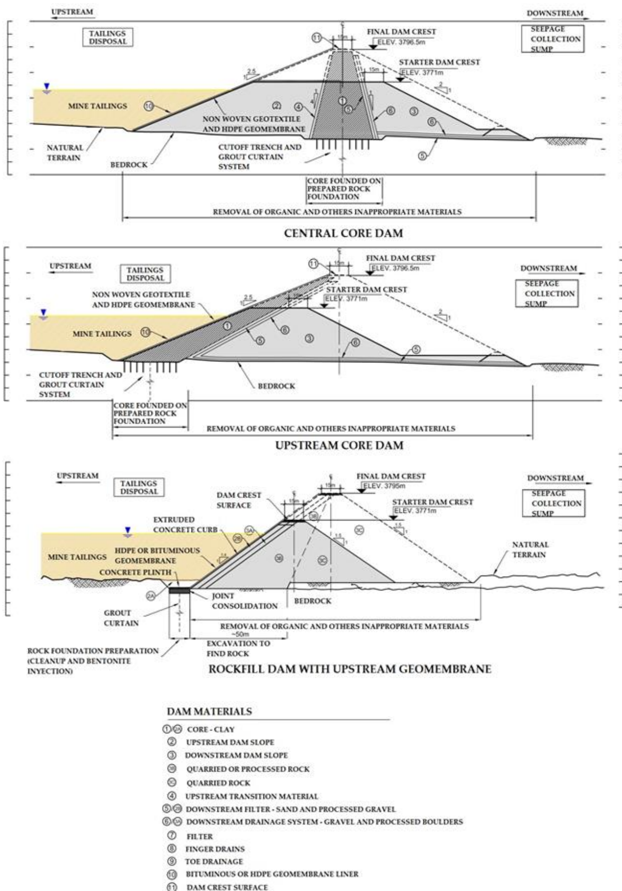
Figure 10. Examples of a geomembrane liner, cutoff trench, and grout curtain system in a TSF.
