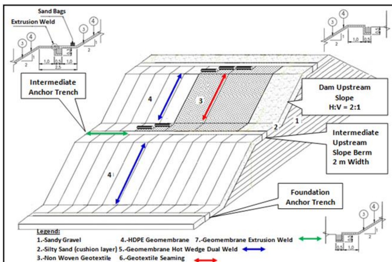
Figure 15. Schematic view of a starter dam with typical geosynthetics installation.
