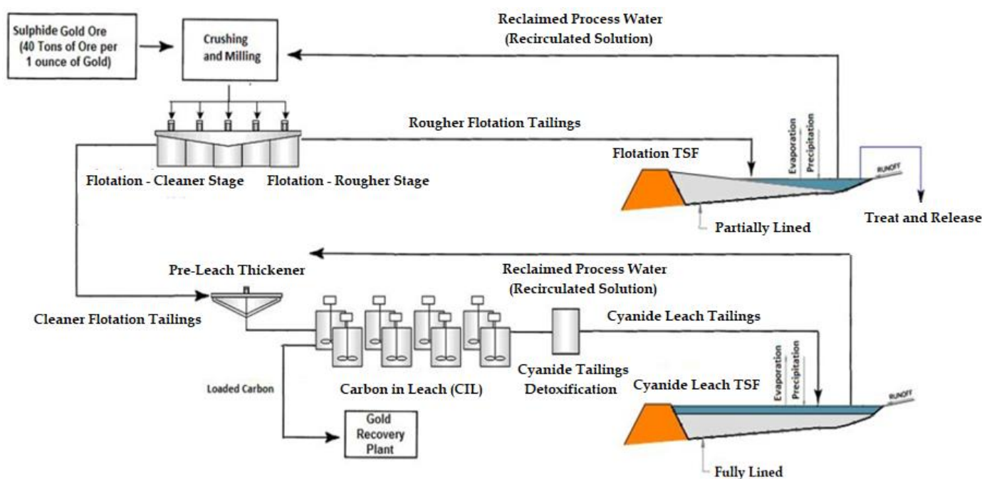
Figure 3. Typical sulphide gold ore flowsheet process—gold mine tailings management [4].
