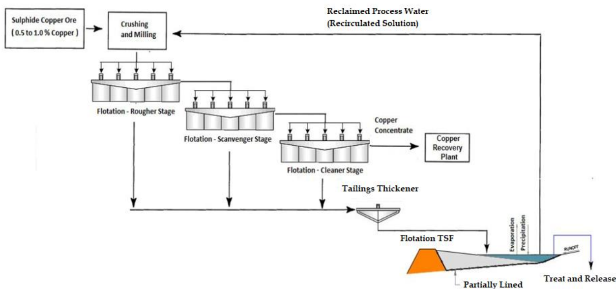
Figure 5. Typical sulphide copper ore flowsheet process—copper mine tailings management [4].
