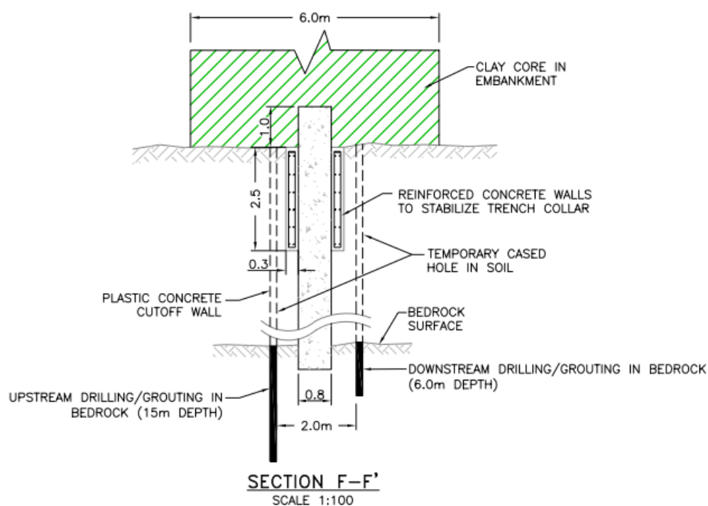
Figure 9. Example of detail of plastic concrete slurry wall with cement–bentonite grout curtain in TSF.
