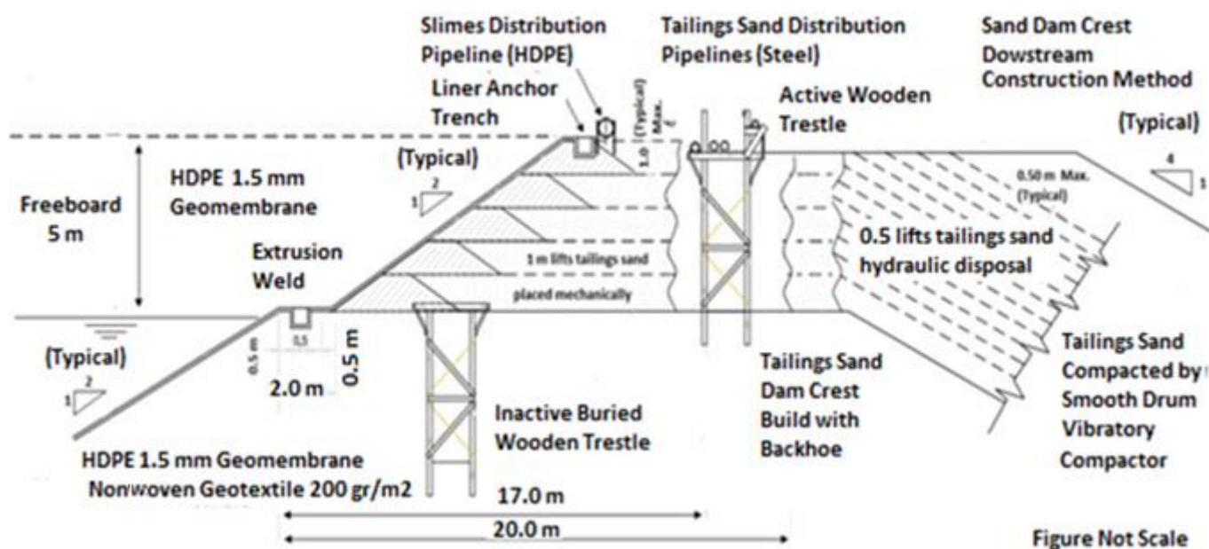
Figure 21. Cycloned tailings sand dam upstream face waterproofing construction detail.
