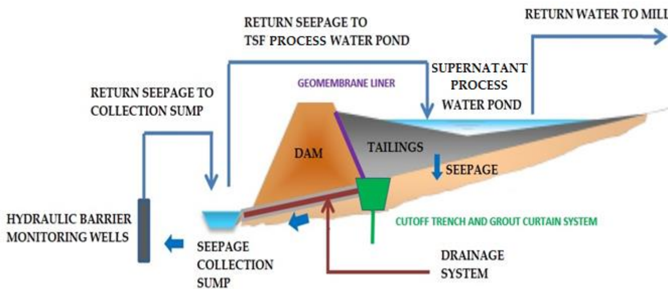
Figure 11. Schematic example of seepage collection system in TSF.
