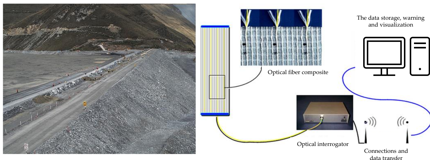
Figure 28. Example of smart geosynthetic with fiber optics technology.
