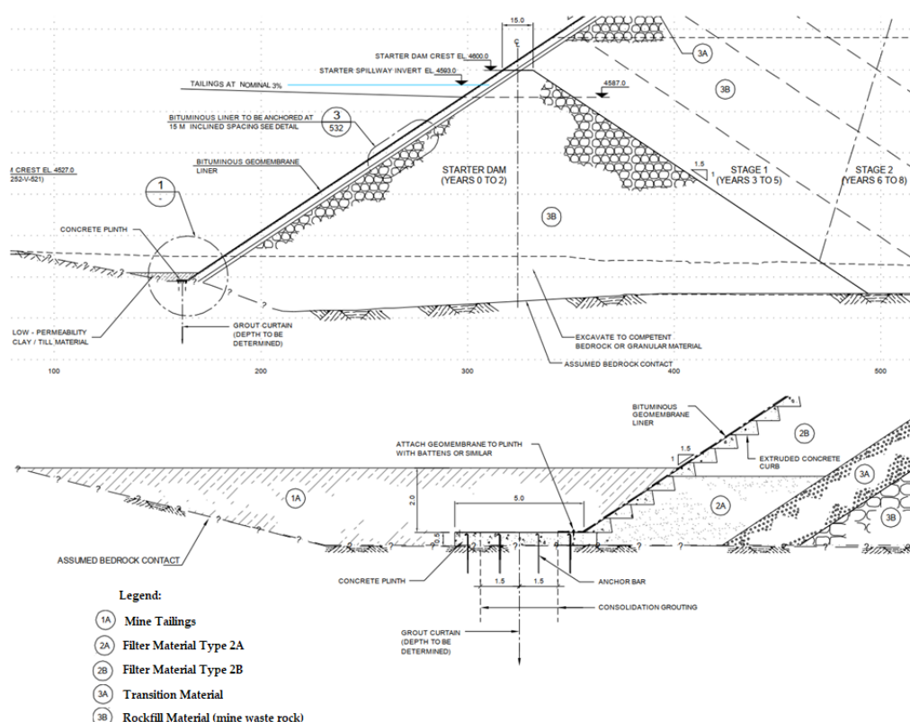
Figure 27. Mine waste rock dam upstream face waterproofing with bituminous geomembrane—construction details.
