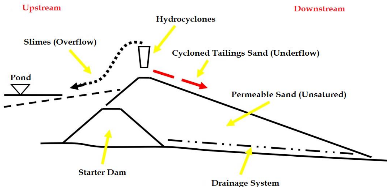
Figure 18. Schematic view of cycloned tailings sand dam construction.
