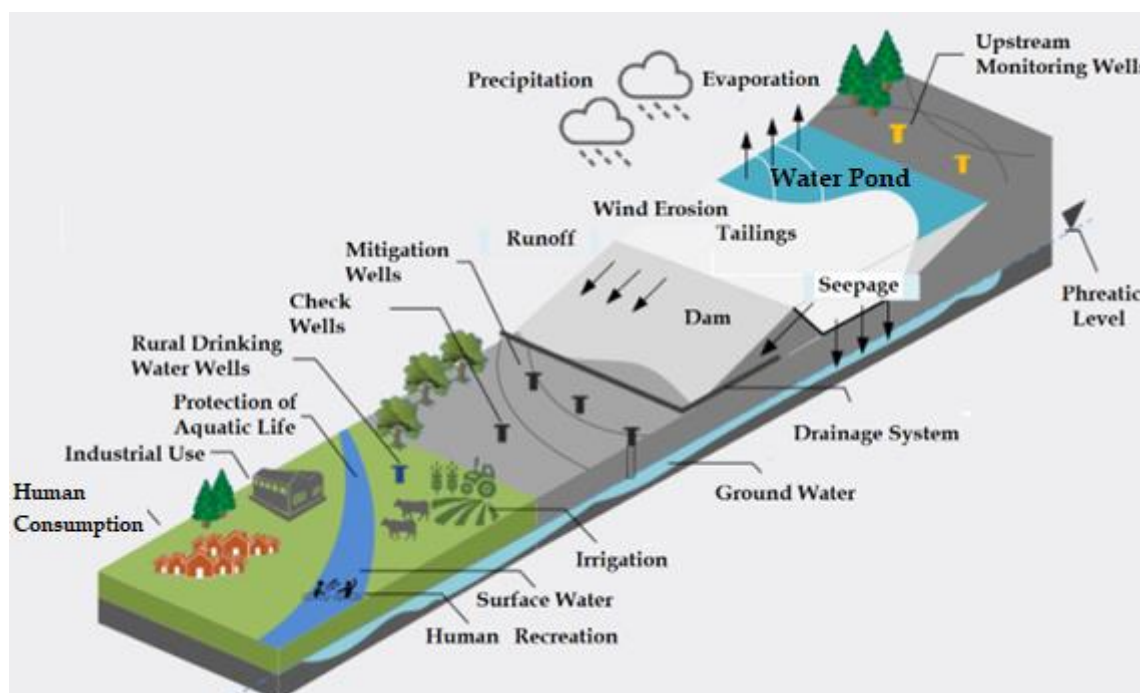
Figure 1. Schematic view of process water (water in contact with mine tailings) management and seepage control in TSF.
