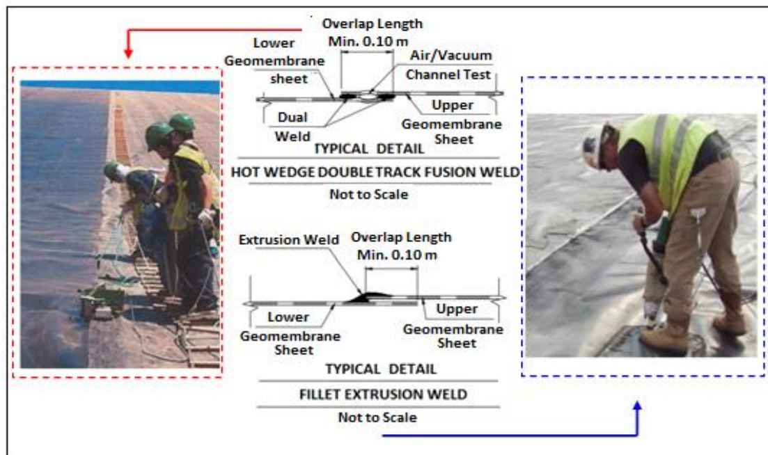
Figure 14. Geomembrane seams—typical details.
