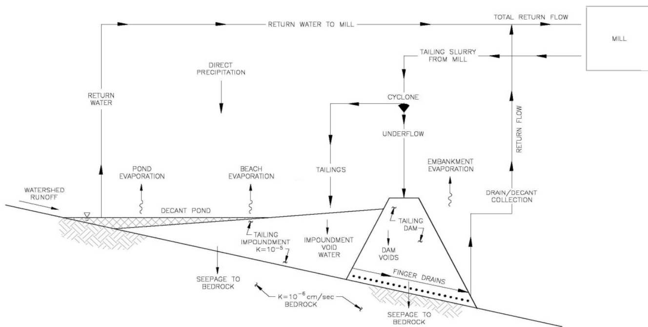
Figure 2. Typical process water management and seepage control in a TSF.
