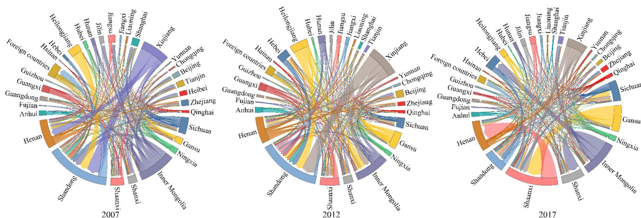
Figure 5. Virtual water flows of the nine provinces in the Yellow River basin, 2007–2017.
