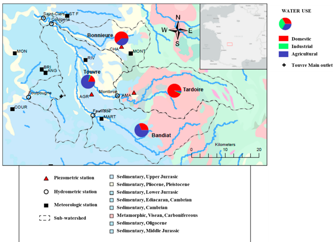
Figure 1. Localisation of the Touvre karst aquifer and of the main hydrological, piezometric and meteorological stations. The percentages of different use of water over the four main sub-catchments (Touvre, Bandiat, Bonnieure and Tardoire) are also mentioned (stations' acronyms: AGR: Agris, AMA: Amant, ANG: Angoulême-Brie-Champoniers, BRI: Brie, CHA: Chazelles, COUR: La Couronne, MART: Marthon, MON: Montignac, MONT: Montembœuf, RIV: Rivières and STF: Saint-Front).
