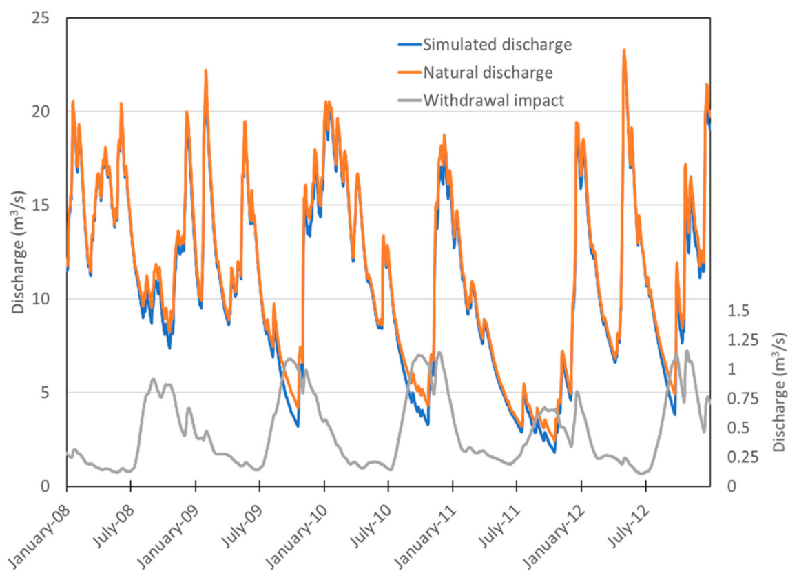
Figure 8. Impact of the naturalization procedure on the discharge at the outlet of the system.
