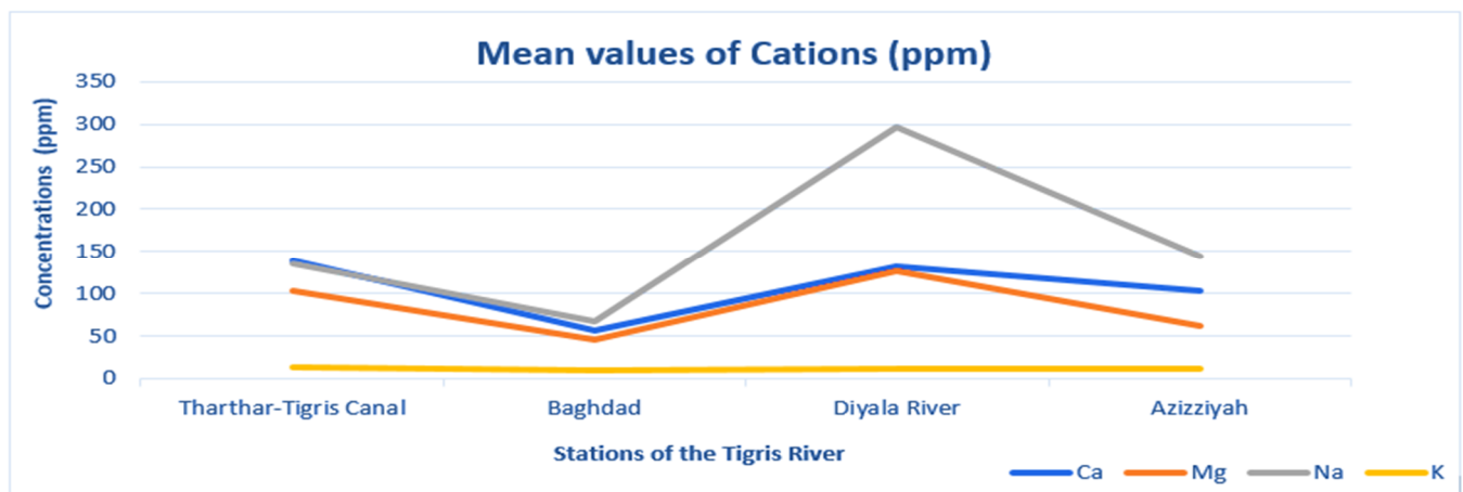
Figure 4. Mean values of annual cations (ppm) along the Tigris River for the period (2005–2020) [26].
