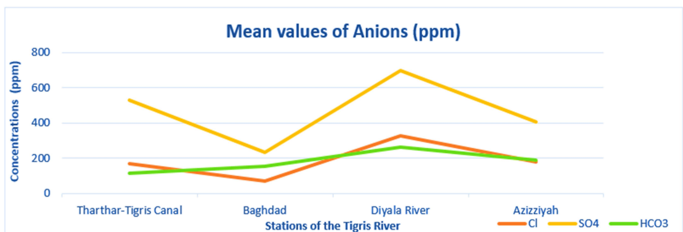
Figure 5. Mean values of annual antions (ppm) along the Tigris River. For the period (2005–2020) [26].
