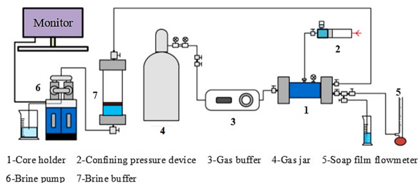
Figure 3. The core flooding experimental process.
