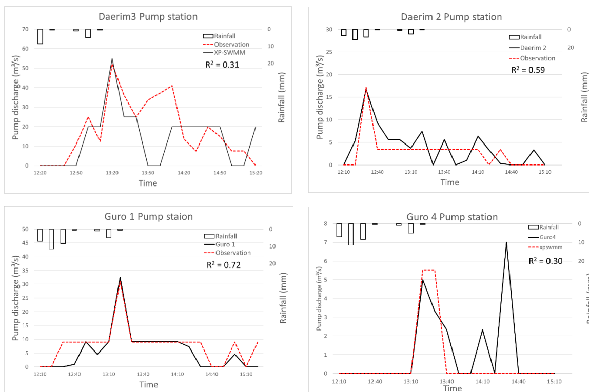
Figure 5. Rainfall-runoff model in Dorim basin by XP-SWMM.
