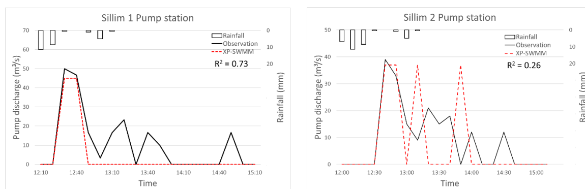
Figure 6. Calibration results of pump station (1 August 2021).
