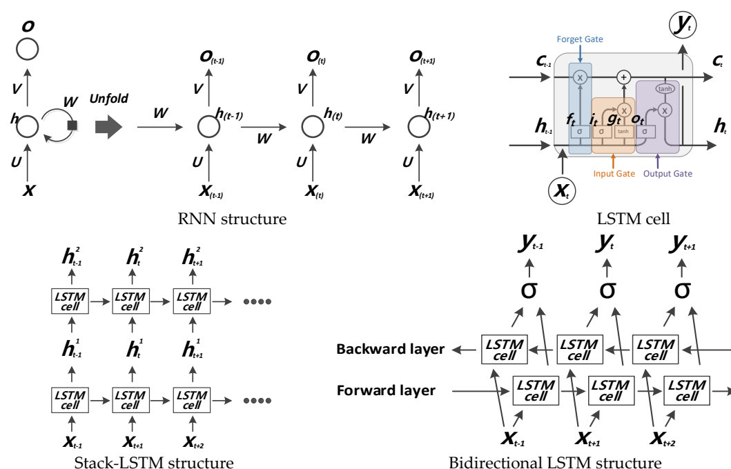
Figure 4. Typical structure of deep learning models.
