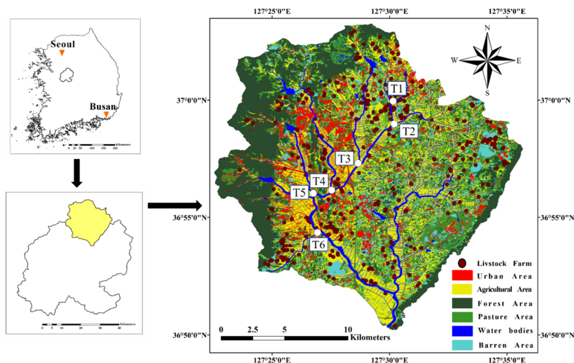
Figure 1. Location of sampling sites in the Miho upstream watershed; white circles indicate the sampling locations (T1 : Naetgeureum Stream, T2 : Dochung Stream, T3 : Sungsan Stream, T4 : Chiljang Stream, T5 : Guam Stream, T6 : Jungsan Stream).
