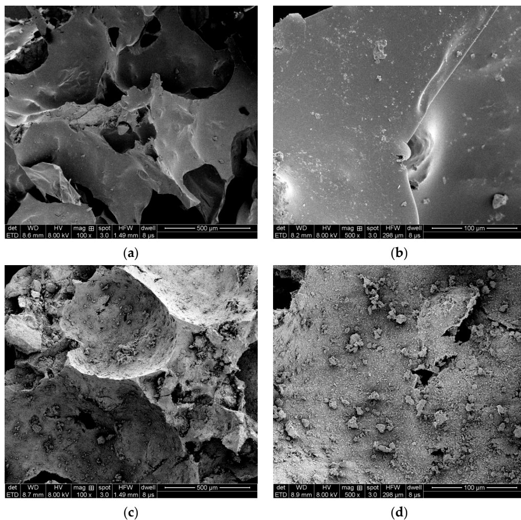
Figure 3. SEM of PU-AL and alum sludge. (a) PU-AL for 100 \times ; (b) PU-AL for 500 \times ; (c) Alum sludge for 100 \times ; (d) Alum sludge for 500 \times .
