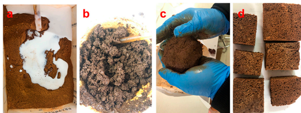
Figure 1. Synthesis of novel alum sludge-based FTWs substrate. (a) alum sludge mixed with organic foaming materials; (b) stirring and forming; (c) granulation; (d) natural drying.
