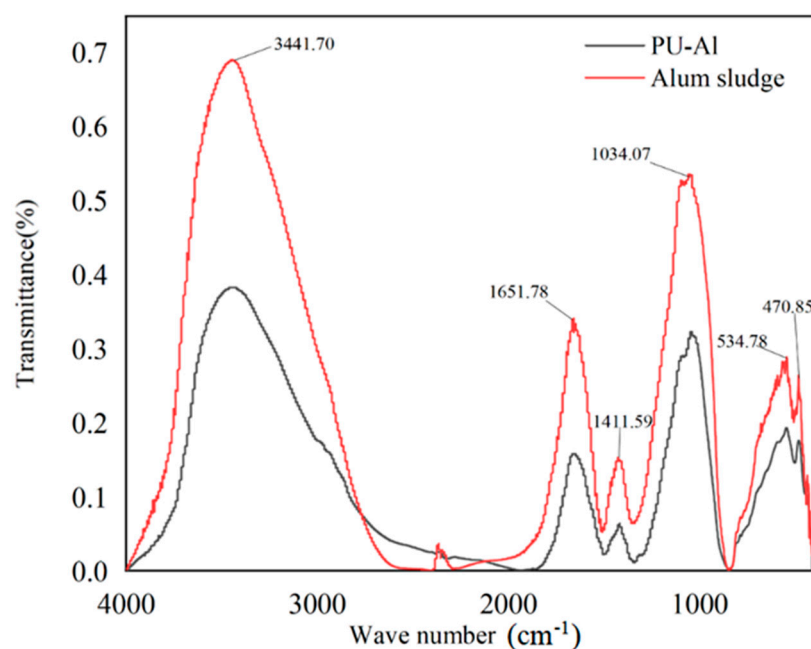
Figure 2. FTIR of PU-AL and alum sludge.
