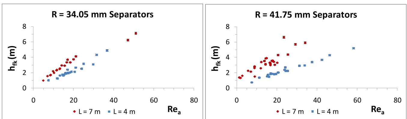
Figure 7. Relationship between the apparent Reynolds number Re_a and the head losses h_{fk} (m) for the separators tested with different helix radiuses R (34.05 mm and 41.75 mm) and tube lengths L (4 and 7 m).
