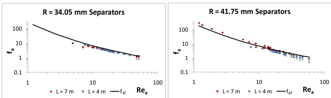
Figure 8. Relationship between the apparent Reynolds number Re_a and the friction factors f_{aI} and f_a for the separators tested with different helix radiuses R (34.05 mm and 41.75 mm) and tube lengths L (4 and 7 m).
