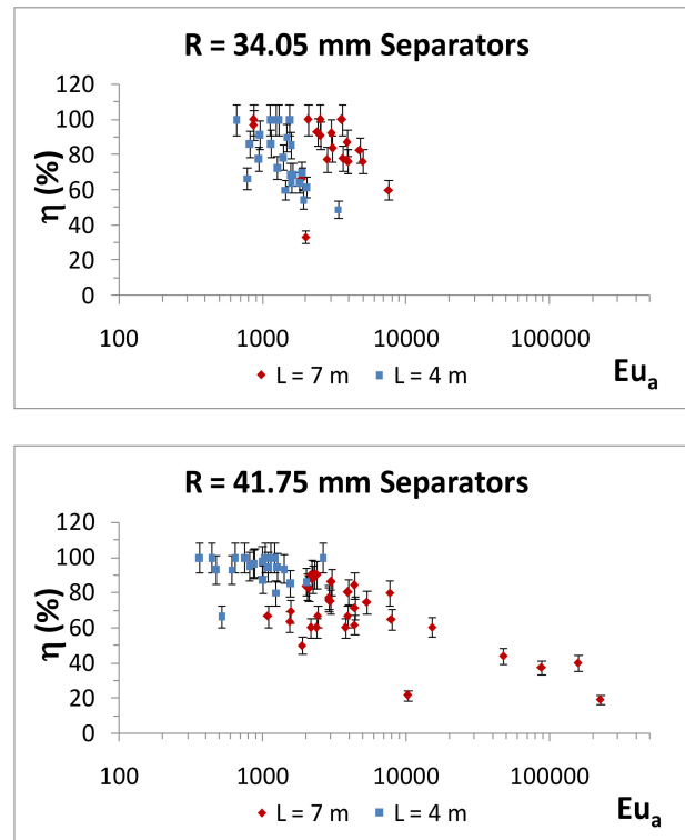
Figure 15. Relationship between apparent Euler number Eu_a and \eta (%) for the separators tested with different helix radii R (34.05 mm and 41.75 mm) and tube lengths L (4 and 7 m).
