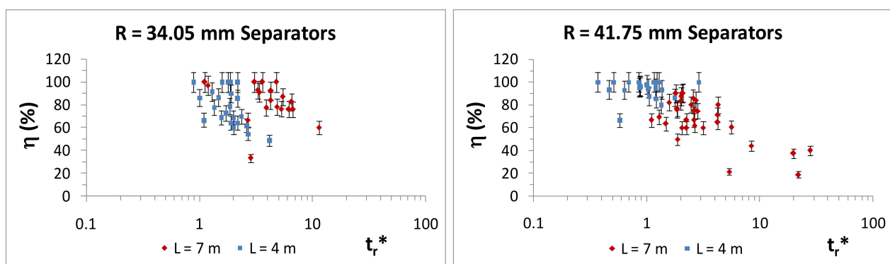
Figure 16. Relationship between t_r^* and \eta (%) for the separators tested with different helix radii R (34.05 mm and 41.75 mm) and tube lengths L (4 and 7 m).
