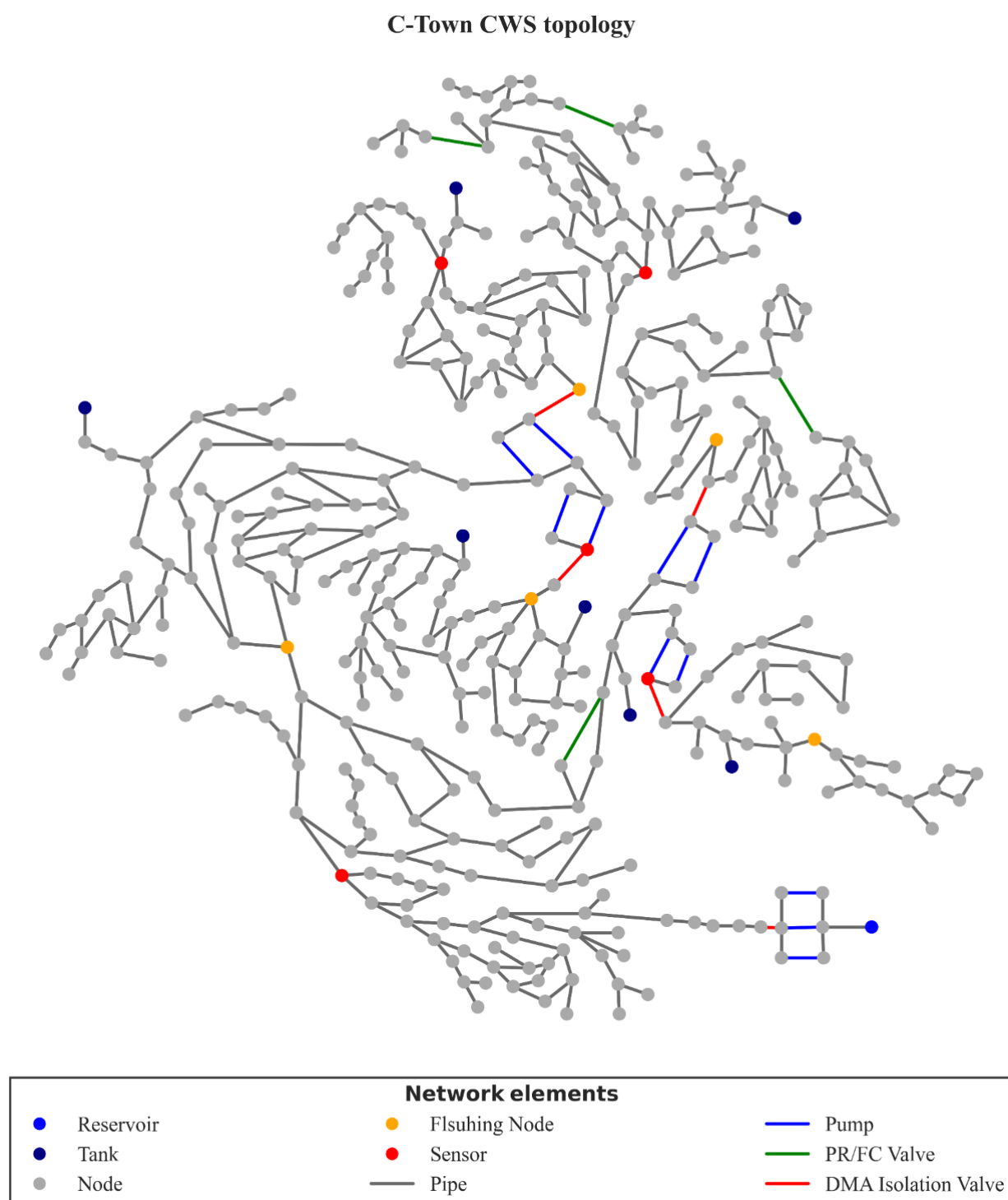
Figure 2. Example of CWS topology for C-Town with a sensor design of five sensors.
