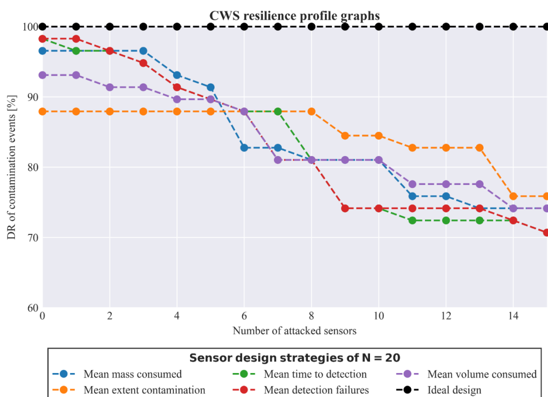
Figure 8. Resilience profile graphs for the five objective functions used to generate topologies of 20 sensors.
