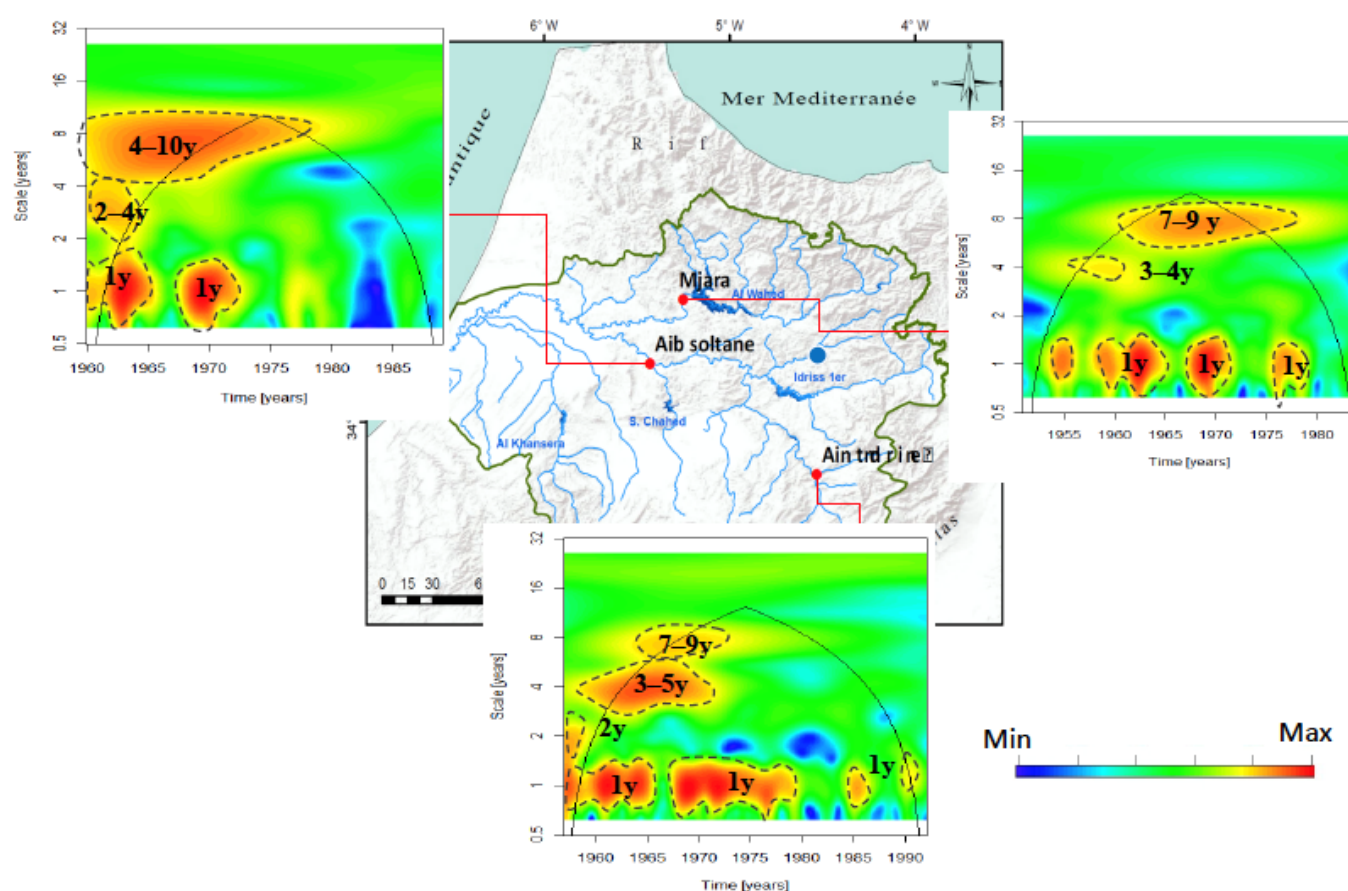
Figure 10. Study of hydrological variability in the Sebou basin.
