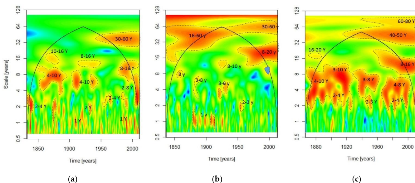
Figure 12. Local spectra of continuous wavelet analysis of climate indices: (a) NAO, (b) SOI, and (c) WMOI.
