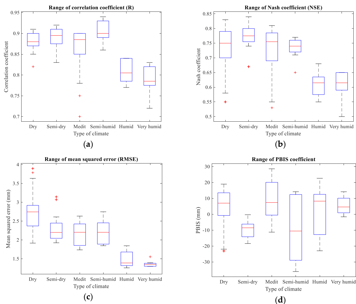
Figure 9. Box plots of statistical coefficients obtained in validation of the two novel methods using data from 32 synoptic weather stations in Iran.
