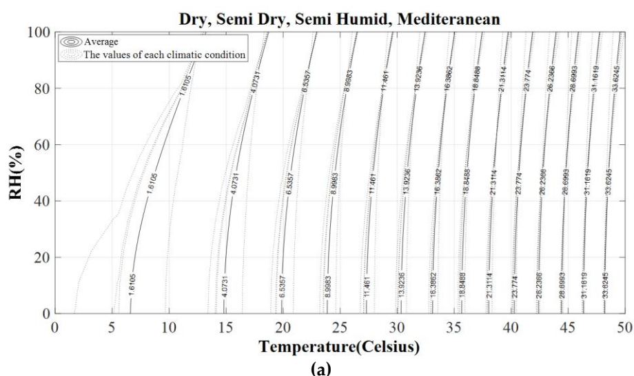
Figure 6. Graphical representation of weights of the six experimental relationships with the two-parameter input combination (a, b, and c, see Table 1) for the six different climate types in Iran.
