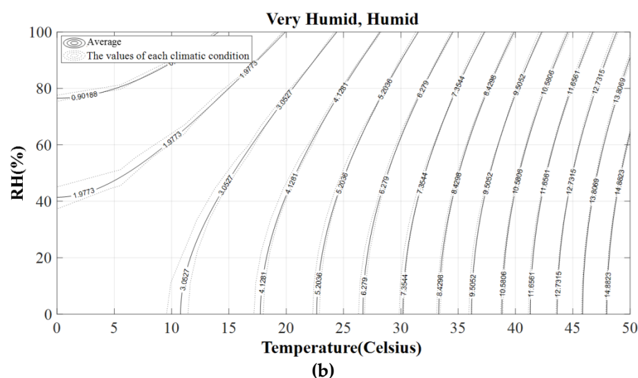
Figure 7. Graphs of the six best experimental relationships (quadratic relationships) simulating pan evaporation with the Table 4. 2. Climatic Correction Coefficients for Climate Types Based on the Basic Relationship (Second Method).
