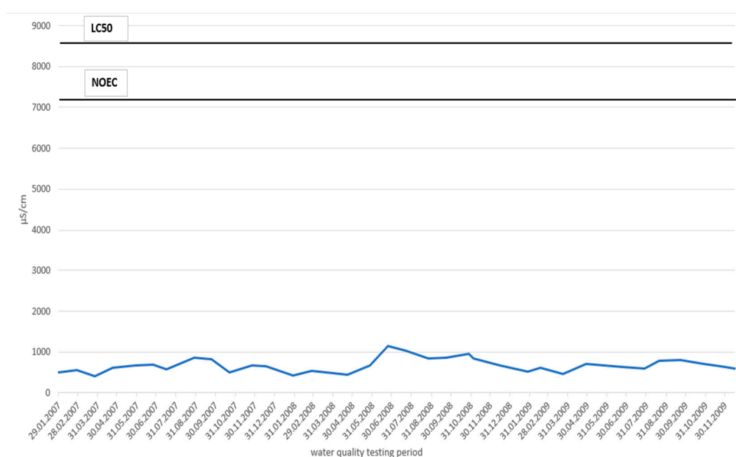
Figure 5. Comparative graph of electrolytic conductivity in the river Długa in 2007–2009 with LC50 and NOEC for Daphnia magna .
