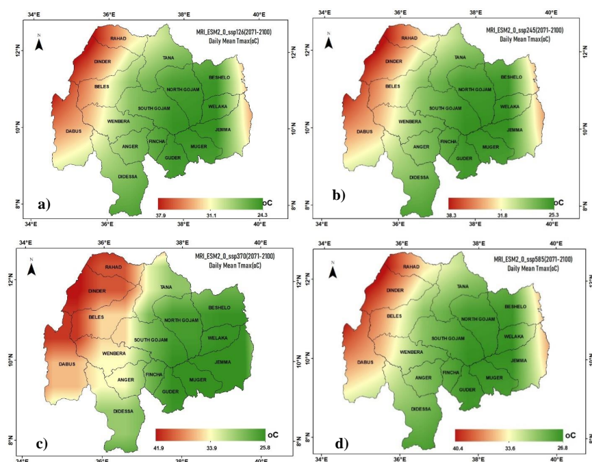
Figure A5. Spatial distribution of CMIP6- MRI-ESM2-0 model daily mean max. temperature (°C) for (a) SSP126(24.3–37.9), (b) SSP245(25.3–38.3), (c) SSP370(25.8–41.9), and (d) SSP585(26.8–40.4) scenarios over the UBNB for the long-term projections (2071–2100). The spatial distributions of mean max. temperature for four SSP scenarios looks identical but the range of the value are different.
