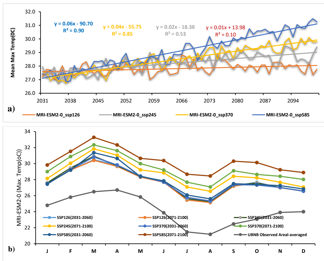
Figure 6. MRI-ESM2-0 model projections under SSP126, SSP245, SSP370, and SSP585 scenario for two future eras (2030s, 2070s). (a) Monthly mean max. temperature (°C) and (b) mean max. temperature (°C) mean annual cycle.
