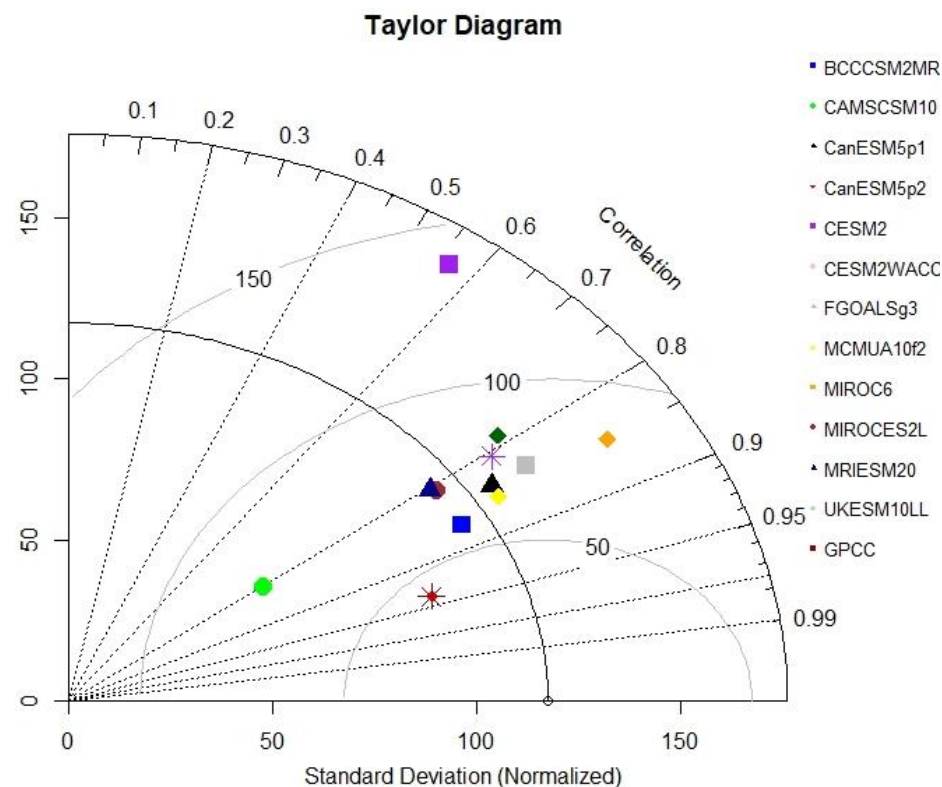
Figure 5. Taylor diagram comparing the temporal performances of twelve CMIP6 models precipitation (mm/day) against the ground-observed and GPCC reanalysis for the baseline period (1981–2010).
