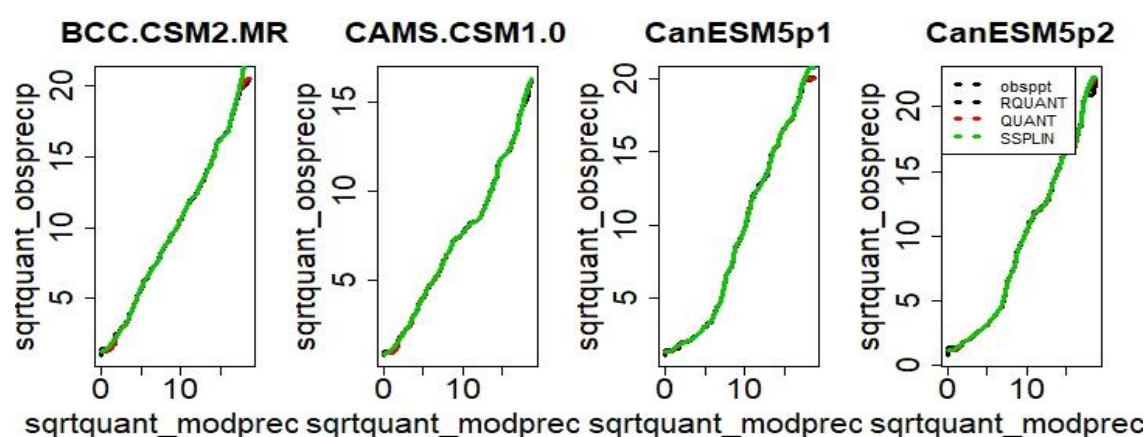
Figure A1. Square root quantile–quantile mapping of model precipitations (BCC-CSM2-MR, CAMS-CSM1.0, CanESM5p1 and CanESM5p2) versus GPCC monthly observation precipitation.
