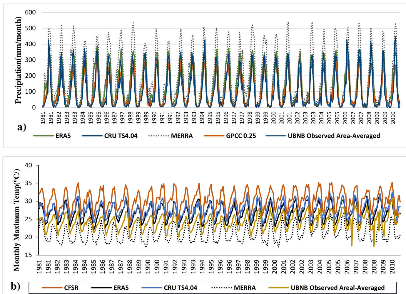
Figure 2. Temporal distribution of monthly observation and reanalysis of (a) precipitation (mm/month), (b) max. temperature (°C/month) within the Upper Blue Nile basin area-averaged.
