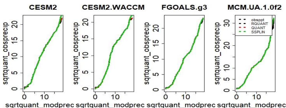
Figure A2. Square root quantile- quantile mapping of model precipitations (CESM2, CESM2-WACCM, FGOALS-g3, and MCM-UA-1.0f2) versus GPCC monthly observation precipitation.
