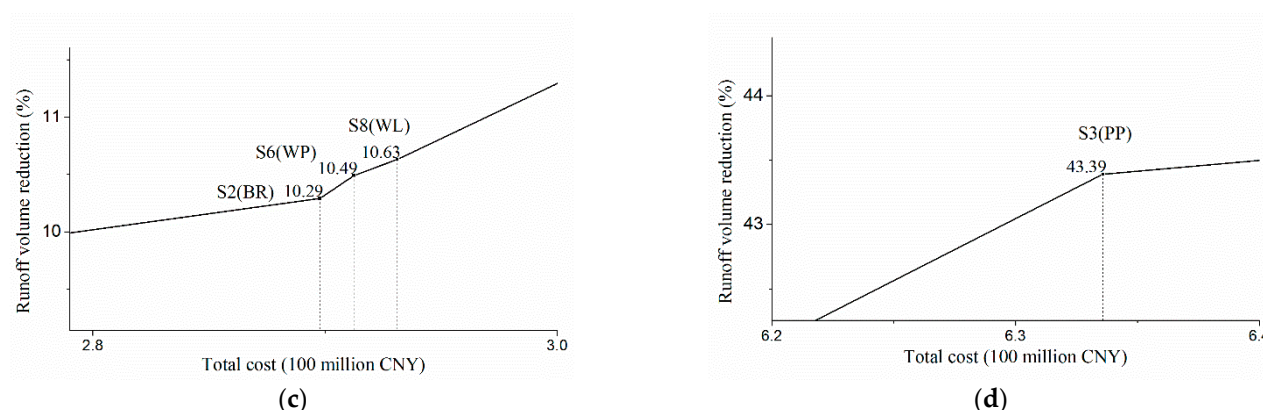
Figure 5. Relationship between total cost and runoff volume reduction with green roofs (GR) and rain cisterns (RC) implemented in series. (b–d) were partial magnifications of (a).
