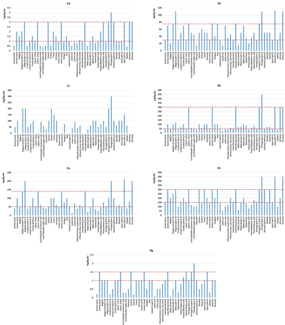
Figure S1. Limits of Heavy Metals for sludge-treated soils (mg/kg dw of soil; Dotted lines: limits proposed by Directive 86/278/EEC).
