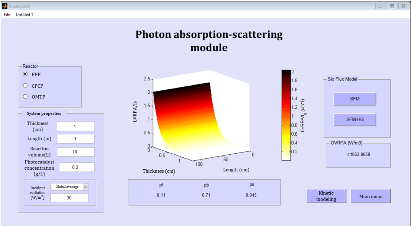
Figure S1. Radiation field simulation of a flat plate photoreactor (FPP) with SFM.
