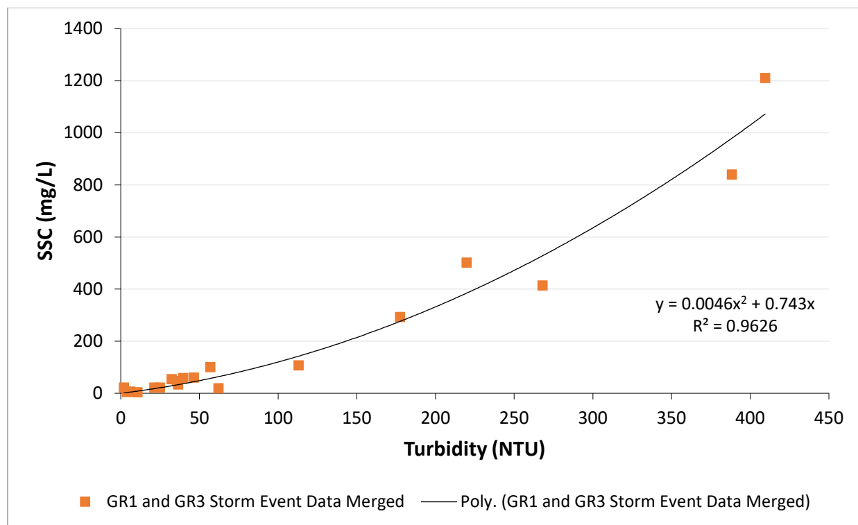
Figure S4: SSC-Turbidity relationship to convert turbidity values to SSC concentrations.
