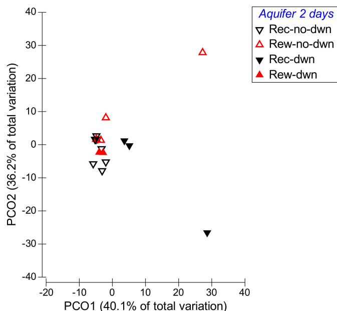
Figure 5. PCoA, for significant PERMANOVA models run for stygobites (2 days: time interval used for calculation of the hydrological phases). Aquifer phase codes as in Table 1.
