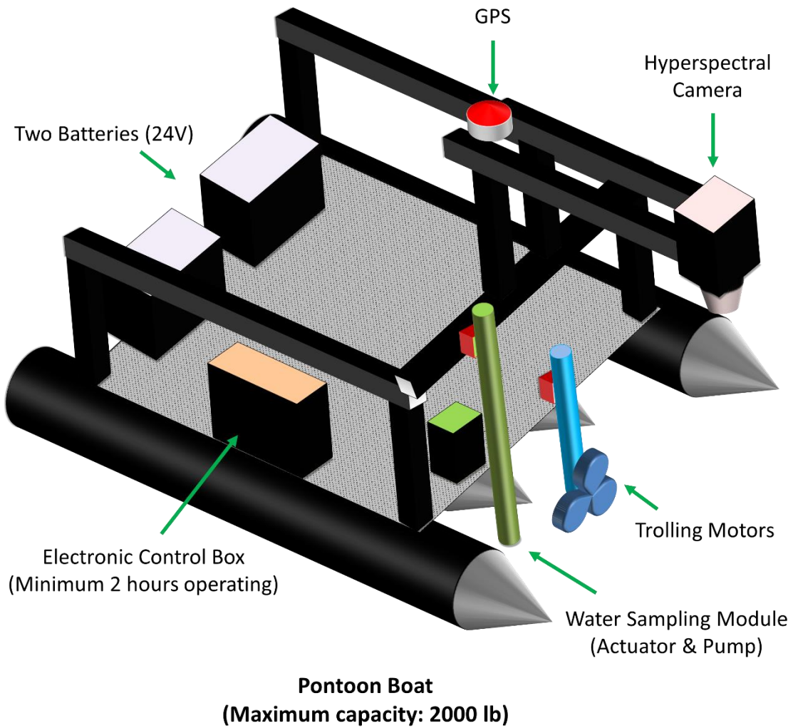
Figure S1: Schematics of the M obile S ampling, S ensing, and H yperspectral I maging Platform (MSSHIP).
