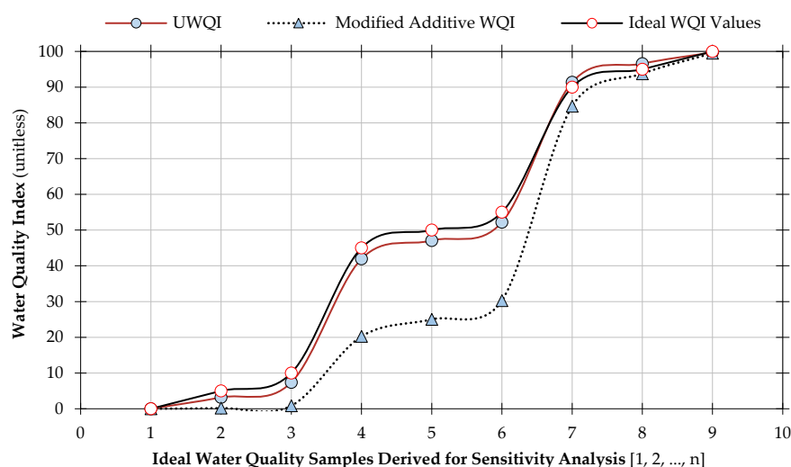
Figure 4. Plot diagram showing the results of the scenario-based analysis of the developed universal water quality index (UWQI) model and the modified additive water quality model against ideal water quality values derived from nine probable scenarios. The nine cases were represented as samples 1, 2, ..., n, which correspond, respectively, to water quality index (WQI) values of 0, 5 and 10 (worst-cases), 45, 50 and 55 (base cases) and 90, 95 and 100 (best cases).
