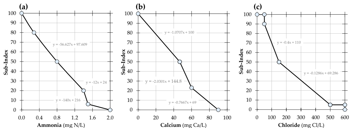
Figure 3. Examples of the graphically established parameter sub-index rating curves for the selected water quality parameters (a) NH_3 , (b) Ca and (c) Cl.
