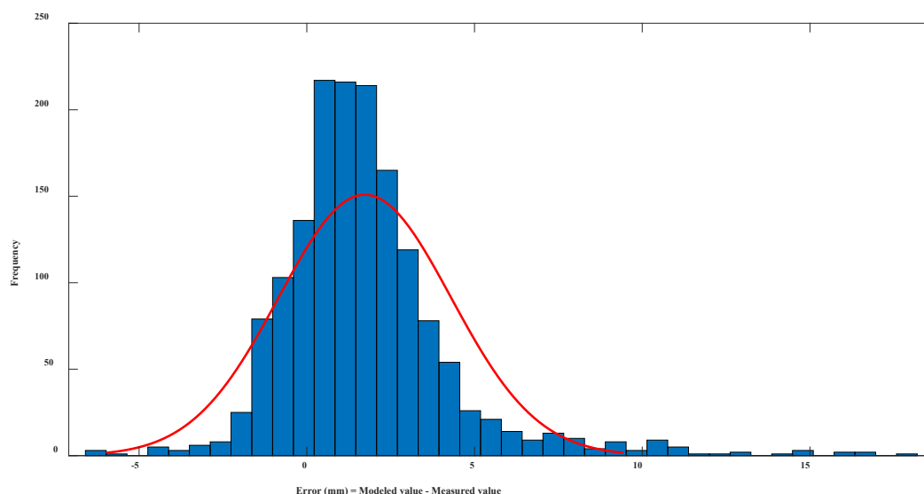
Figure 10. Error distribution of model 2 in the validation period. The red line represents the fitted normal distribution.
