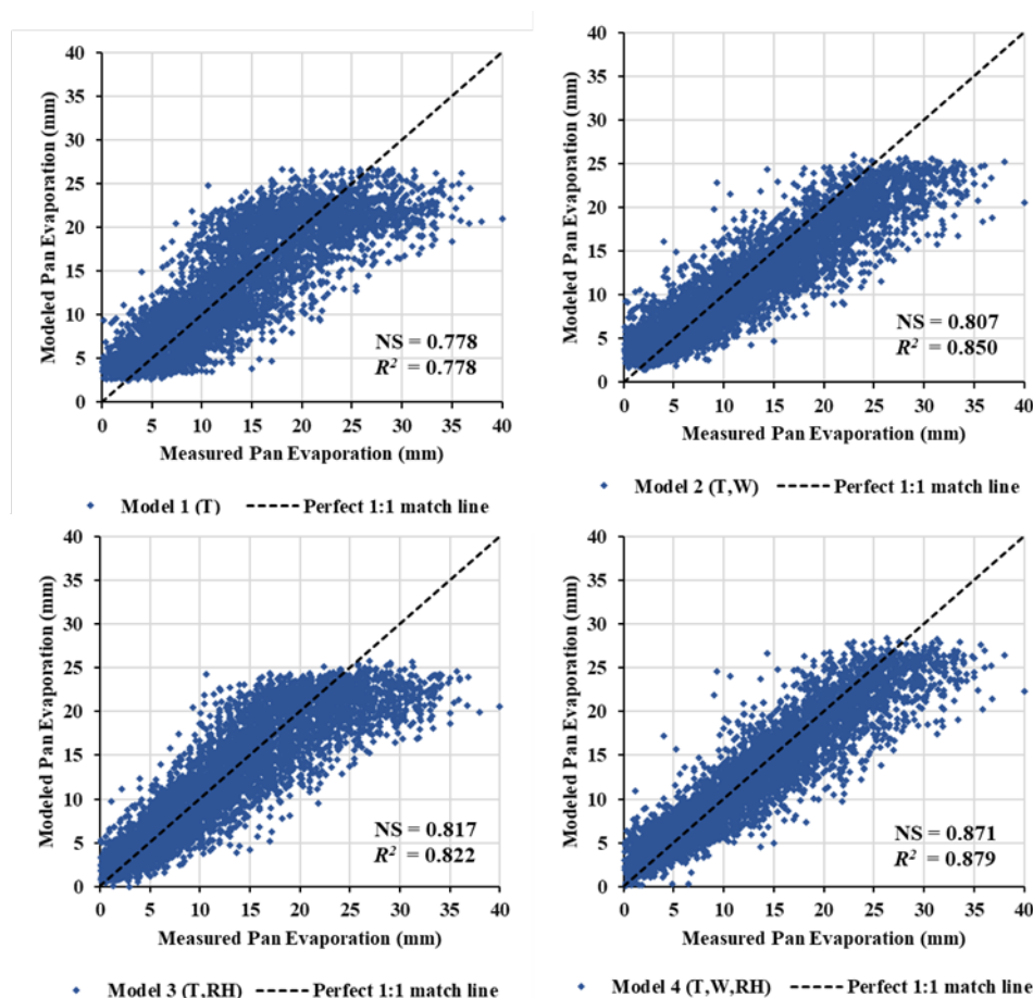
Figure 5. Modeled versus measured pan evaporation depths (mm) for the training period at KIA weather station. T: average daily temperature; RH: average relative humidity; W: average wind speed.
