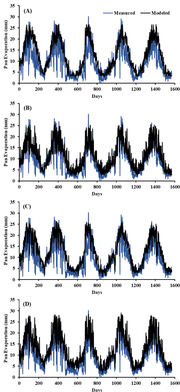
Figure 7. Modeled and measured pan evaporation time series (validation period) for (A) Model 1 (T), (B) Model 2 (T, W), (C) Model 3 (T, RH), and (D) Model 4 (T, W, RH). T: average daily temperature; RH: average relative humidity; W: average wind speed.
