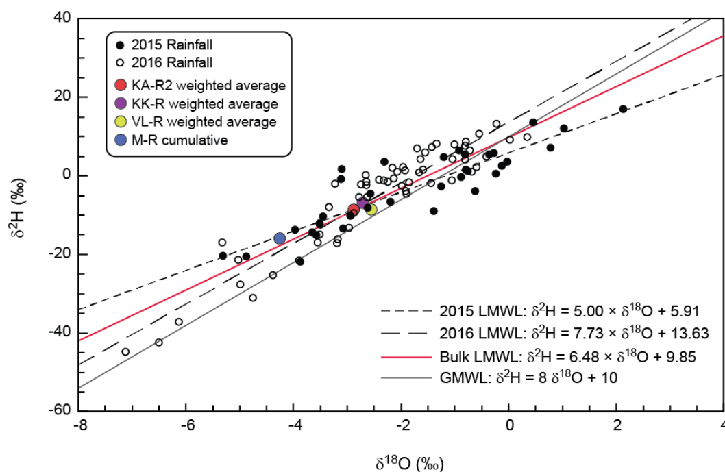
Figure 6. \delta^{18}\text{O} vs. \delta^2\text{H} plot showing distribution of rainwater samples and slope of local meteoric water lines defined for both 2015 and 2016 as well a combined local meteoric water line. The weighted averages for the rainwater collectors over the sampling period are also shown. LMWL: local meteoric water line; GMWL: global meteoric water line.
