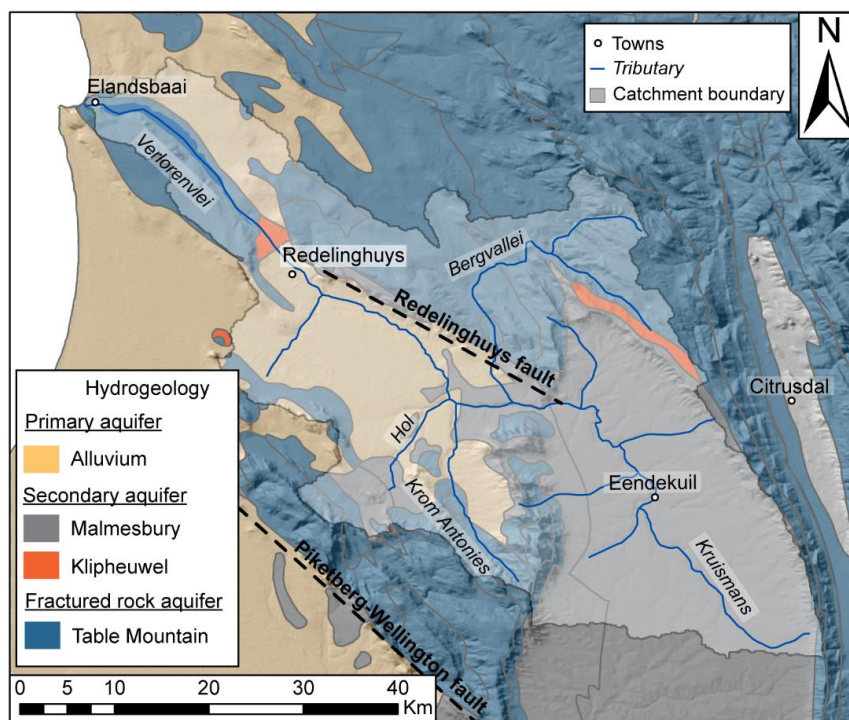
Figure 2. Geology and hydrogeology of the Verlorenvlei catchment.
