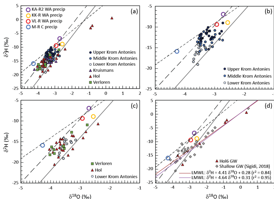
Figure 8. Stable isotope values of groundwater from the Verlorenvlei catchment. (a) Groundwater from all four tributaries examined in this study as well as the weighted average of precipitation from the four precipitation collectors, (b) variation between the upper, middle and lower Krom Antonies, (c) comparison between the Hol and lower Krom Antonies groundwater, and (d) comparison between the groundwater from location Hol6 and shallow groundwater in the alluvial aquifer in the Hol and down to the confluence derived from [38]. LMWLs for 2015 and 2016 as per Figure 6. GMWL (solid grey line) derived from Craig (1961). WA = weighted average, precip = precipitation, GW = groundwater.
