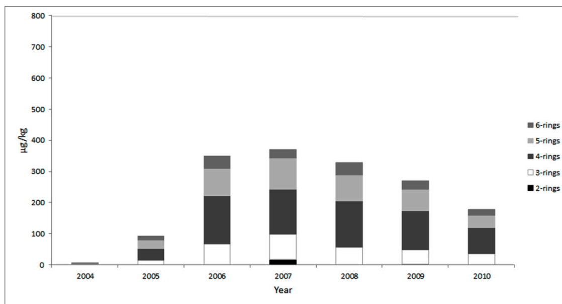
Figure 3. Annual average of polycyclic aromatic hydrocarbons (PAHs) ( \Sigma 16 PAHs in \mu\text{g/kg} ) for 2004 to 2010 ( n = 4 ) and group profiles of LPAHs (two or three-fused rings) and of HPAHs (four to six-fused rings) in the sediments from Sacca di Goro. The EQS limit (Good/Moderate) for the sum of PAHs according to the WFD is indicated.
