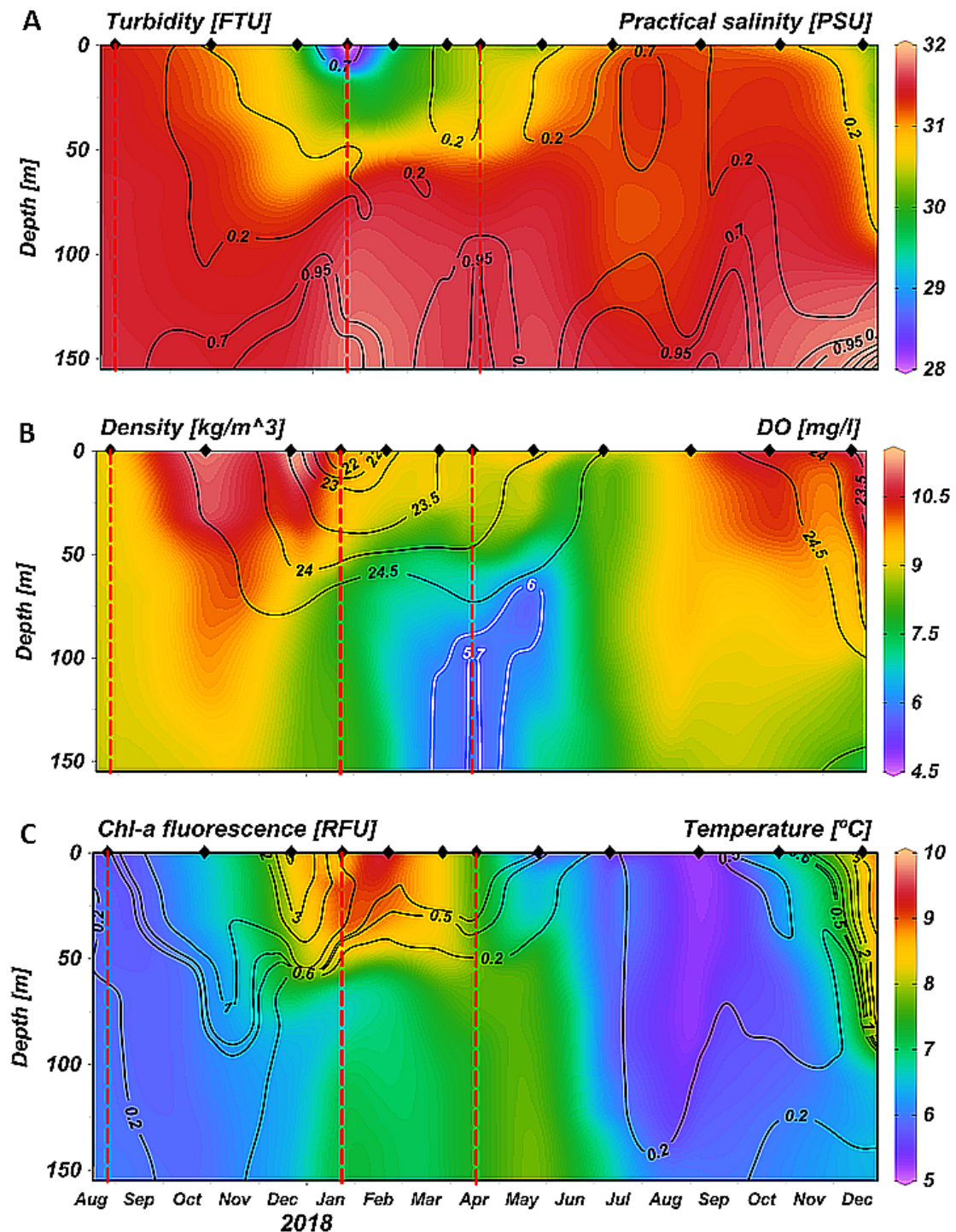
Figure 2. Time series at the fixed station over the entire water column measured between August 2017 and December 2018 of (A) salinity (in gradient color) and turbidity (black isolines); (B) dissolved oxygen (in gradient color and white isolines) and density anomaly (black isolines); and (C) temperature (in gradient color) and Chl-a fluorescence (black isolines). The enhanced observation period: red dotted lines are the field trips of August 2017, January 2018, and April 2018.
