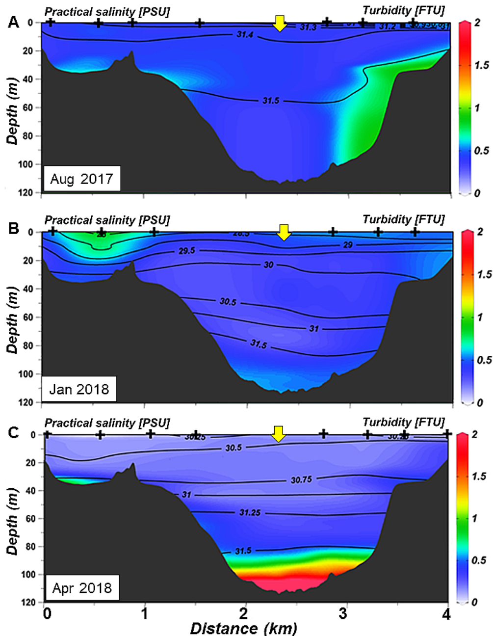
Figure 4. Cross-bay section of turbidity (color gradient) and salinity (isolines) for (A) August 2017; (B) January 2018; and (C) April 2018. The intersection between cross-bay and along-bay sections is marked with a yellow arrow.
