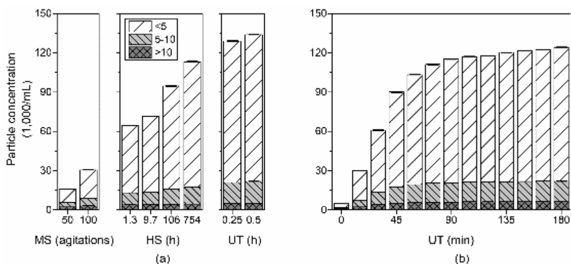
Figure 4. (a) Particle concentration of batch A during manual shaking (MS), horizontal shaking (HS) and ultrasonic treatment (UT). (b) Particle concentration of batch A (20 mg/L PS particles) during ultrasonic treatment (UT) for 180 min. Particles in all diagrams were grouped in size fractions <5 \mu\text{m} , 5–10 \mu\text{m} and >10 \mu\text{m} . Error bars show standard deviation of n = 3 .
