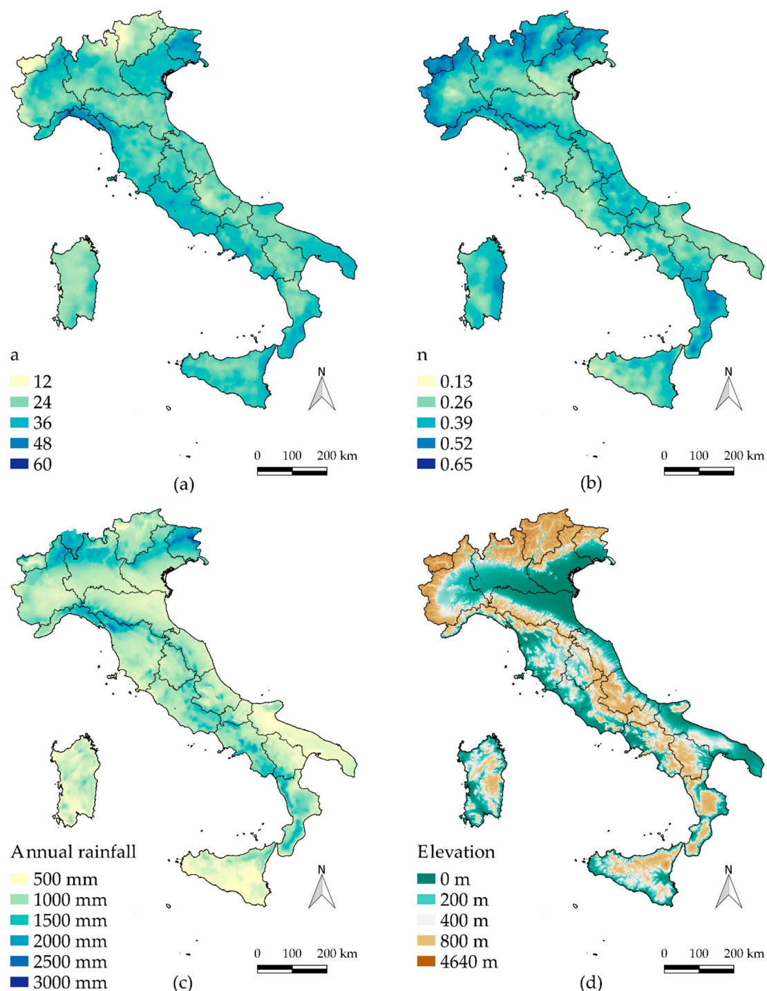
Figure 7. Parameters a (a) and n (b) of the DDF curves evaluated on the basis of the data contained in I 2 -RED. The maps are characterized by a 1 \times 1 km spatial resolution. (c) Mean annual precipitation as mapped by [26]. (d) Elevation data, Shuttle Radar Topography Mission (SRTM) digital elevation model.
