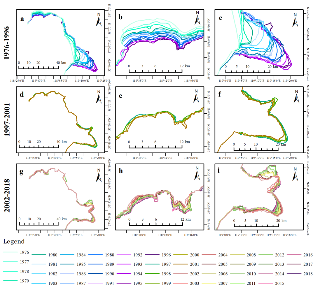
Figure S2. Spatiotemporal dynamic distributions of the coastline in the whole YRD (a,d,g), the northern coast (b,e,h) and the Yellow River Estuary (c,f,i) from 1976 to 2018.
