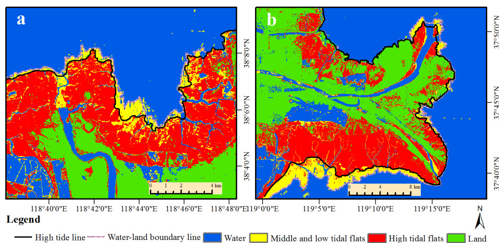
Figure S1. Extraction of the high tide line and water-land boundary line from the remote sensing classification for 2013.
