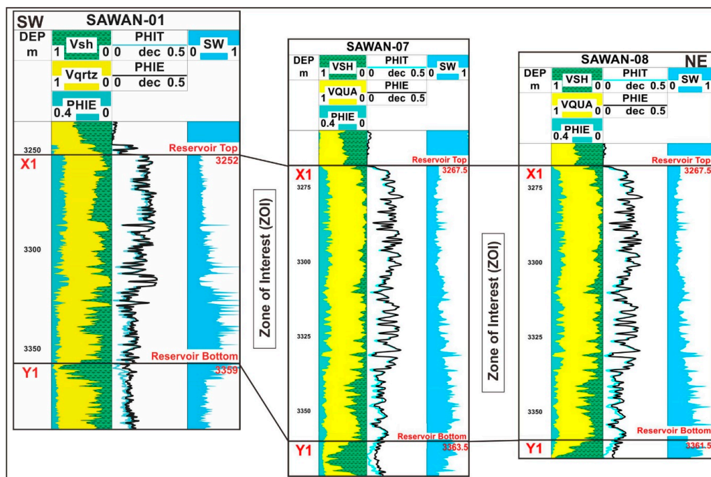
Figure 6. The structural configuration of study wells highlighting the thicknesses of the reservoir parameters within the ZOI.
