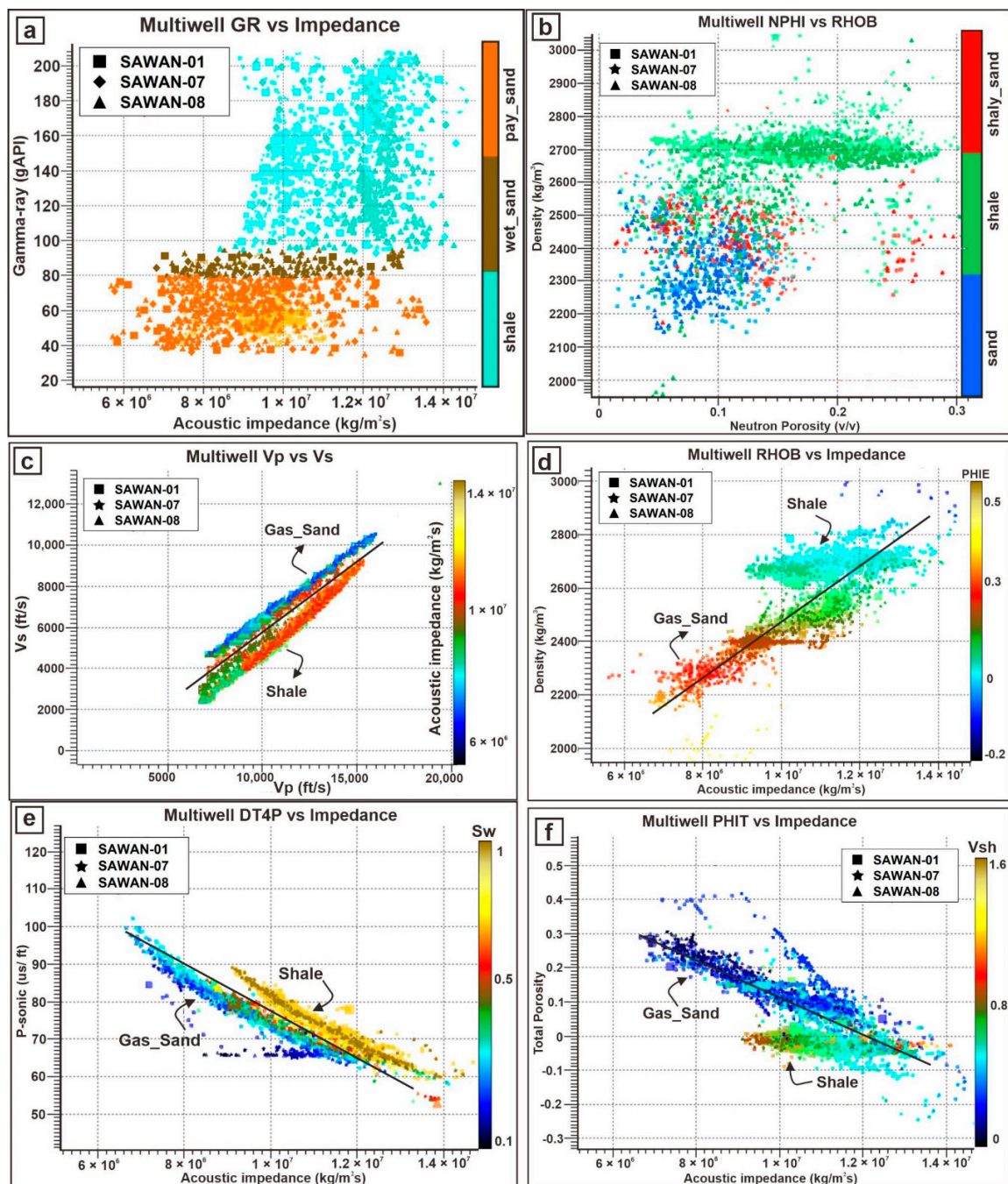
Figure 16. Facies discrimination analysis using AI and facies logs cross-plots. (a) GR-AI cross-plot color-coded with generated shale-wet_sand-pay_sand facies log showing the cutoff values for gas-sand (pay-sands) and shaly-sand (wet-sands) and shale sediments. (b) Neutron-Density cross-plot color-coded with extracted 3Lithos facies log showcasing the sand and intermixing of shaly-sand and shale facies. The mixing of thin-laminated fine-grained shaly-sand and shale facies shows scattered plotting. (c) V_s - V_p cross-plot color-coded with AI log highlighting good separation of gas-sand and shale facies. (d) RHOB-AI cross-plot color-coded with effective porosity log displays reliable discrimination of porous gas-sand facies versus non-porous shale facies. (e) P-sonic-AI cross-plot color-coded with S_w distinguishing the clean sand and shale facies. (f) Total Porosity-AI cross-plot color-coded with V_{sh} highlights excellent discrimination of porous gas-saturated sand facies and non-porous shale facies.
