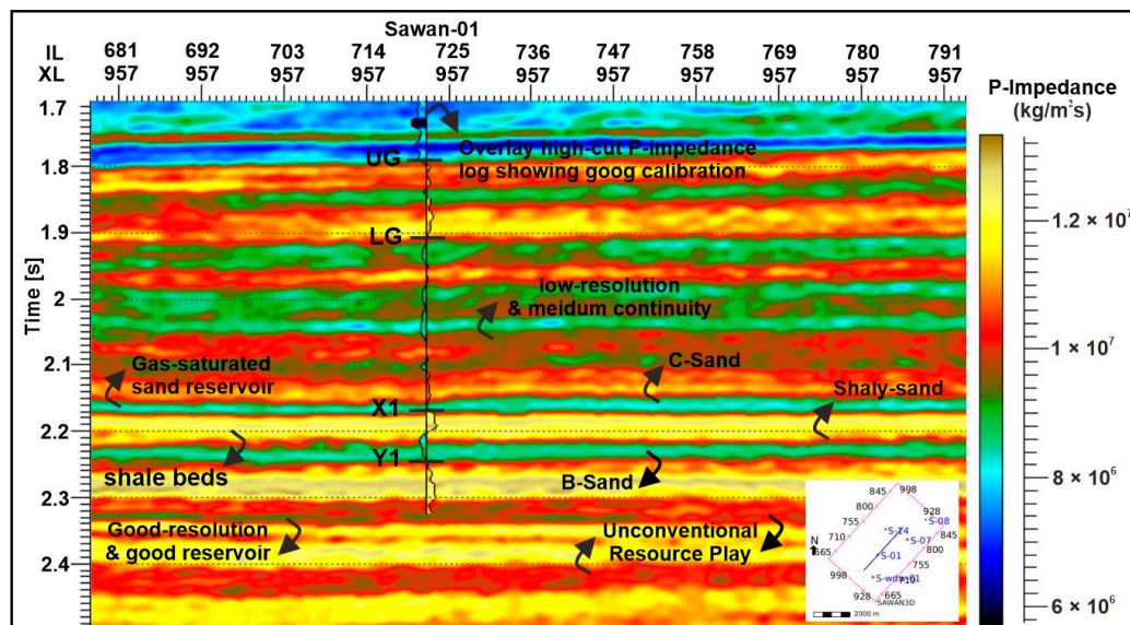
Figure 10. Overly of p-impedance log on inverted AI section at S-01 well and crossline-957 location.
