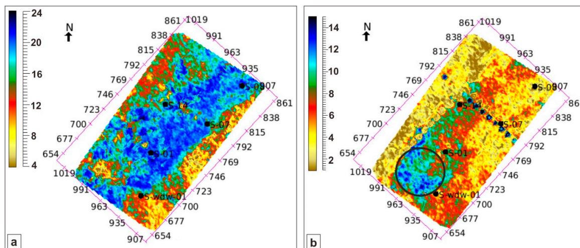
Figure 13. Porosity distribution maps of (a) C-sand interval and (b) B-sand interval. The black circle shows the high porosity region with no drilled well and can be exploited for future drillings.
