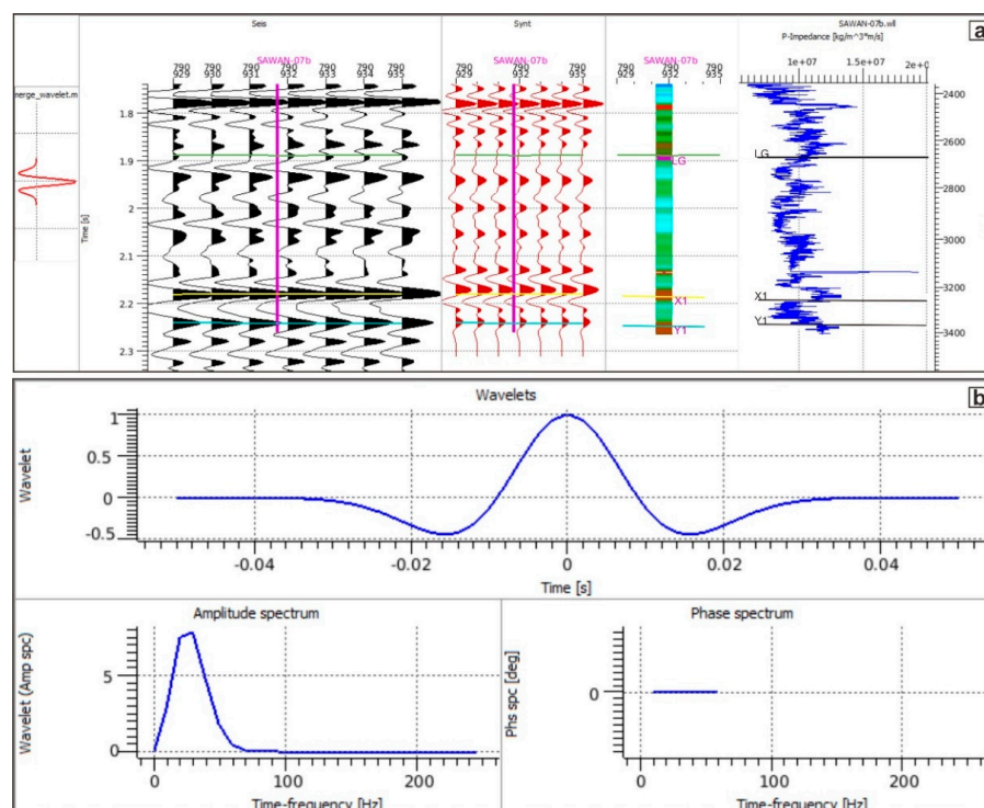
Figure 7. (a) Seismic-to-well tie among synthetic and seismic traces of S-07. X1 and Y1 horizons show the ZOI. (b) Average wavelet extracted along with amplitude and phase spectrum for study wells.
