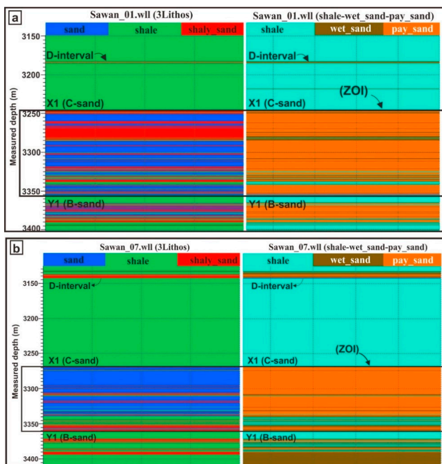
Figure 15. Facies log created for LGF using GR log to differentiate the sand (blue), shale (green), and the shaly_sand (red) facies (left side). Whereas, facies log generated using GR and resistivity (LLD) log to differentiate the pay-sands (orange), wet-sands (brown), and shale (cyan) facies (right side) for (a) S-01, and (b) S-07.
