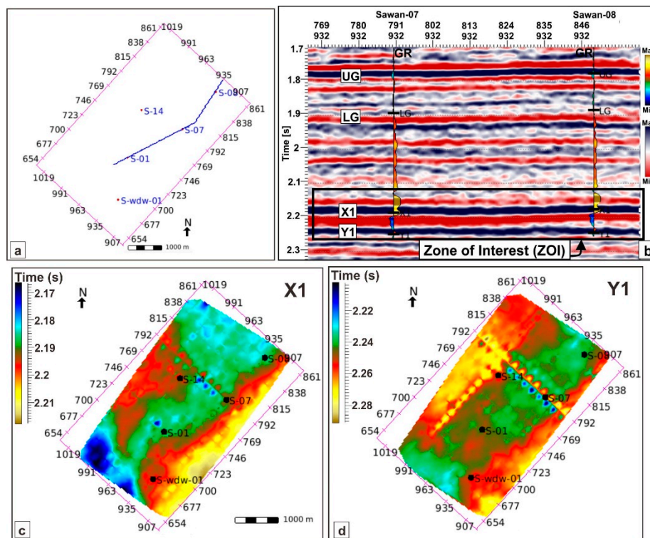
Figure 3. (a) Basemap of the study area. The arbitrary line is selected that is passing through S-01, S-07, and S-08 wells, which were used for inversion analysis. (b) Seismic-to-well-tie of S-07 and S-08 at crossline-932. The black rectangle highlights the targeted area. (c) Interpolation of the X1 (C-sand) horizon. (d) Interpolation of the Y1 (B-sand) horizon.
