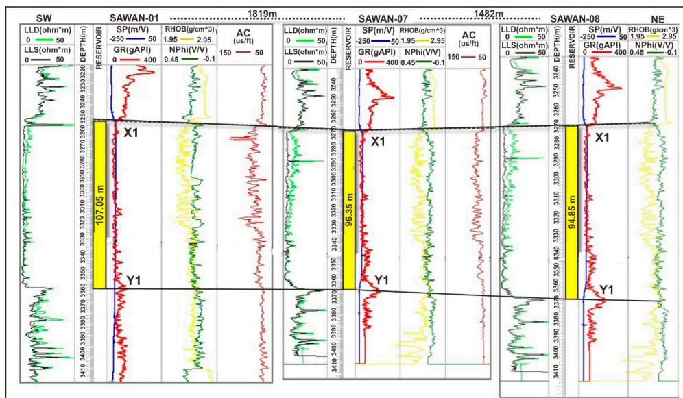
Figure 5. Stratigraphic correlation of study wells showing the thicknesses of ZOI in the study area.
