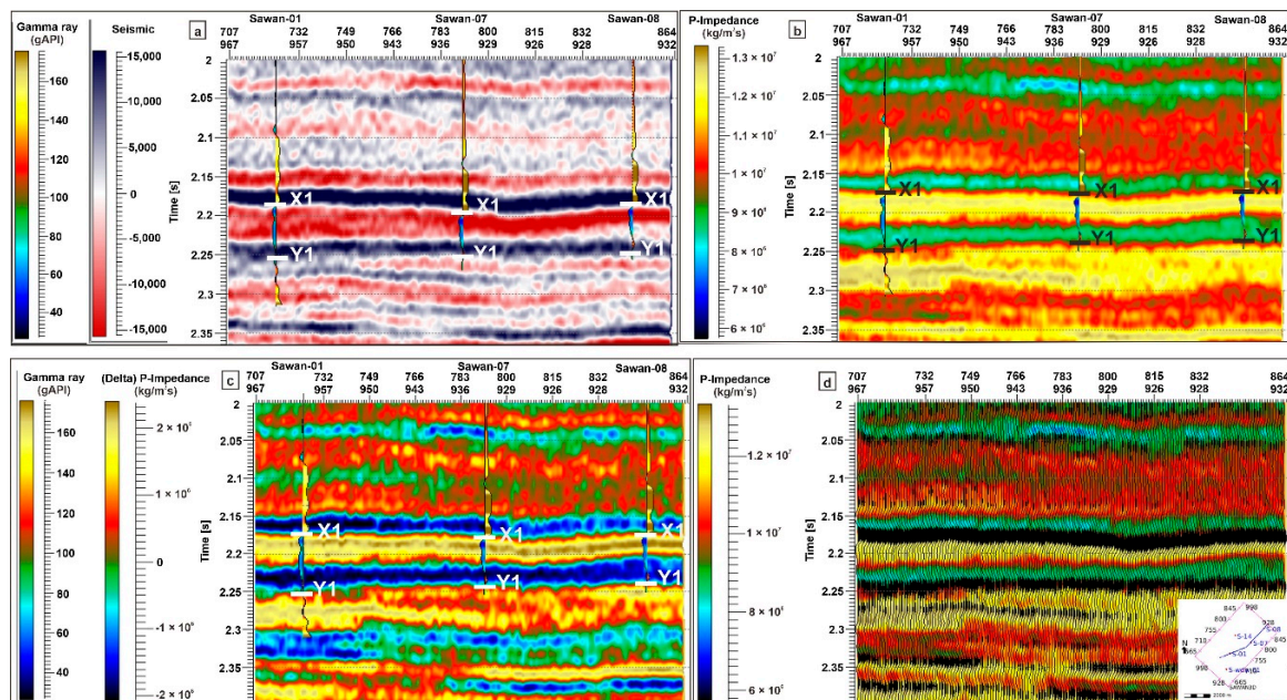
Figure 9. Well-tops, overlay GR (API) log, and S-01, S-07, S-08 wells on (a) a seismic section. (b) Inverted AI broadband model. (c) Inverted AI broadband model with well-tops, overlay GR (API) log, and S-01, S-07, S-08 wells. (d) Overlay of seismic section (wiggle) and inverted broadband AI model that shows the same resolution.
