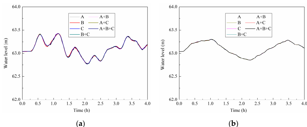
Figure 11. Water level variation process concerning locations of hydropower stations. (a) Lower lock head of the ship lift; (b) Approach channel entrance.
