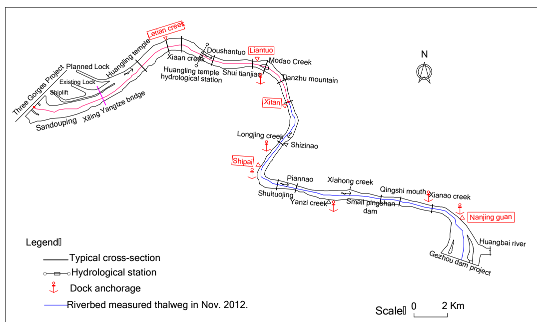
Figure 2. Schematic of river channel between the Three Gorges Dam (TGD) and the Gezhouba Dam (GZD).
