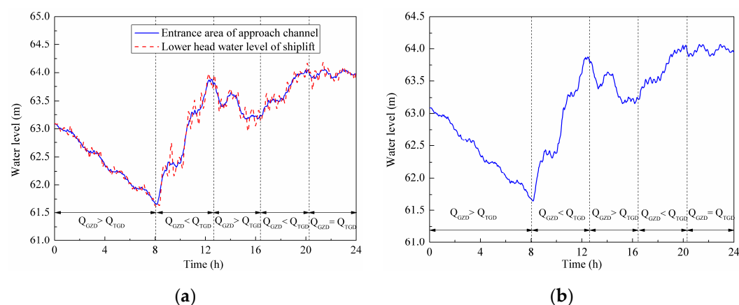
Figure 17. Water level variation process regarding double-peak regulation. (a) Approach channel entrance and lower lock head of the ship lift; (b) The planned approach channel entrance.
