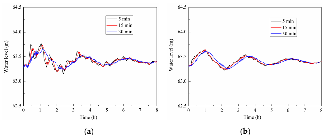
Figure 10. Water level variation process with regulation time. (a) Lower lock head of the ship lift; (b) Approach channel entrance.
