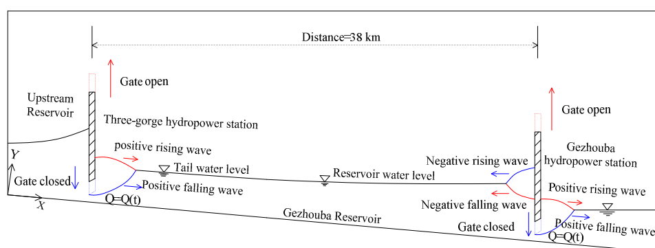
Figure 12. Schematic diagram of the Three Gorges and Gezhouba cascade hydropower station.
