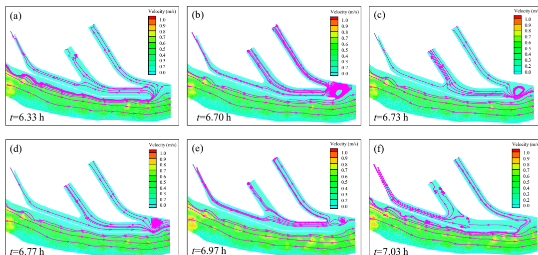
Figure 15. The typical streamline and velocity in multi-approach channels under single-peak regulation of hydropower stations. (a) t=6.33 h; (b) t=6.70 h; (c) t=6.73 h; (d) t=6.77 h; (e) t=6.97 h; (f) t=7.03 h.
