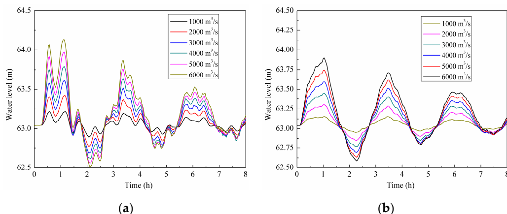
Figure 9. Water level variation process with flow variation amplitude. (a) Lower lock head of the ship lift; (b) Approach channel entrance.
