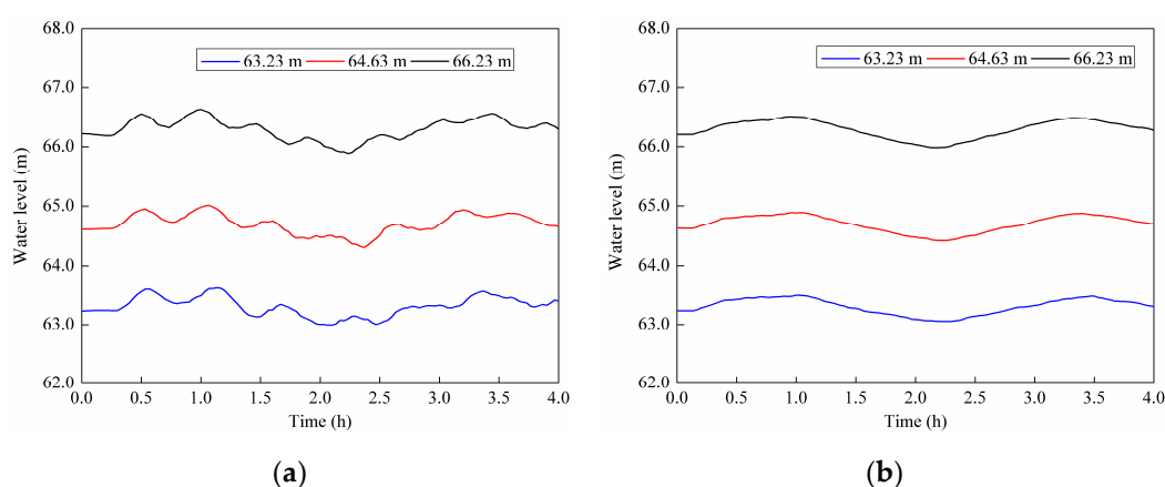
Figure 7. Water level variation process with initial water surface elevation. (a) Lower lock head of the ship lift; (b) Approach channel entrance.
