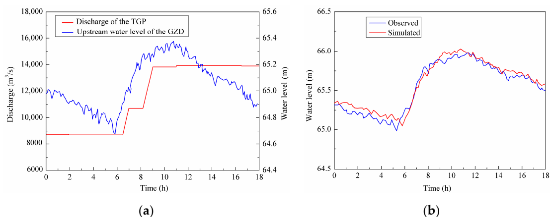
Figure 5. Boundary conditions and simulation results using a one-dimensional model. (a) Boundary conditions; (b) Comparison of the observed and simulated water level at the lower lock head of the ship lift.
