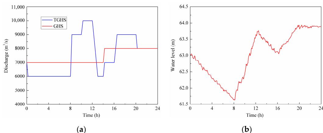
Figure 16. Boundary conditions. (a) Daily regulation between the TGHS and GHS; (b) Water level at the Xitan Station.
