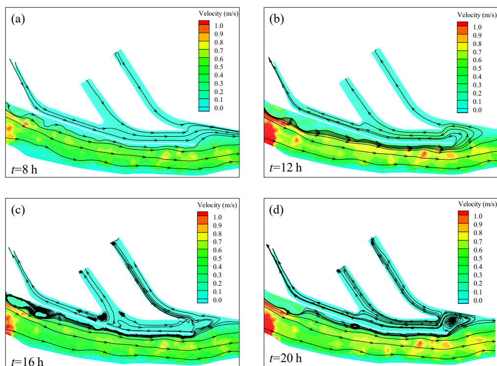
Figure 18. The typical streamline and velocity in multi-approach channels under double-peak regulation of hydropower stations. (a) t = 8 \text{ h} ; (b) t = 12 \text{ h} ; (c) t = 16 \text{ h} ; (d) t = 20 \text{ h} .
