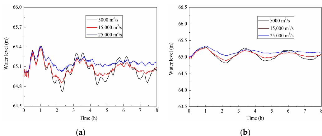
Figure 8. Water level variation process with the base flow. (a) Lower lock head of the ship lift; (b) Approach channel entrance.
