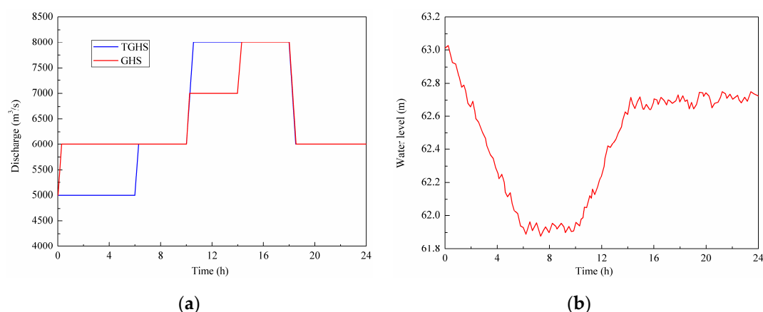
Figure 13. Computation boundary. (a) Flow process of the Three Gorges Hydropower Station (TGHS) and the Gezhouba Hydropower Station (GHS); (b) Water level at the Xitan Station.
