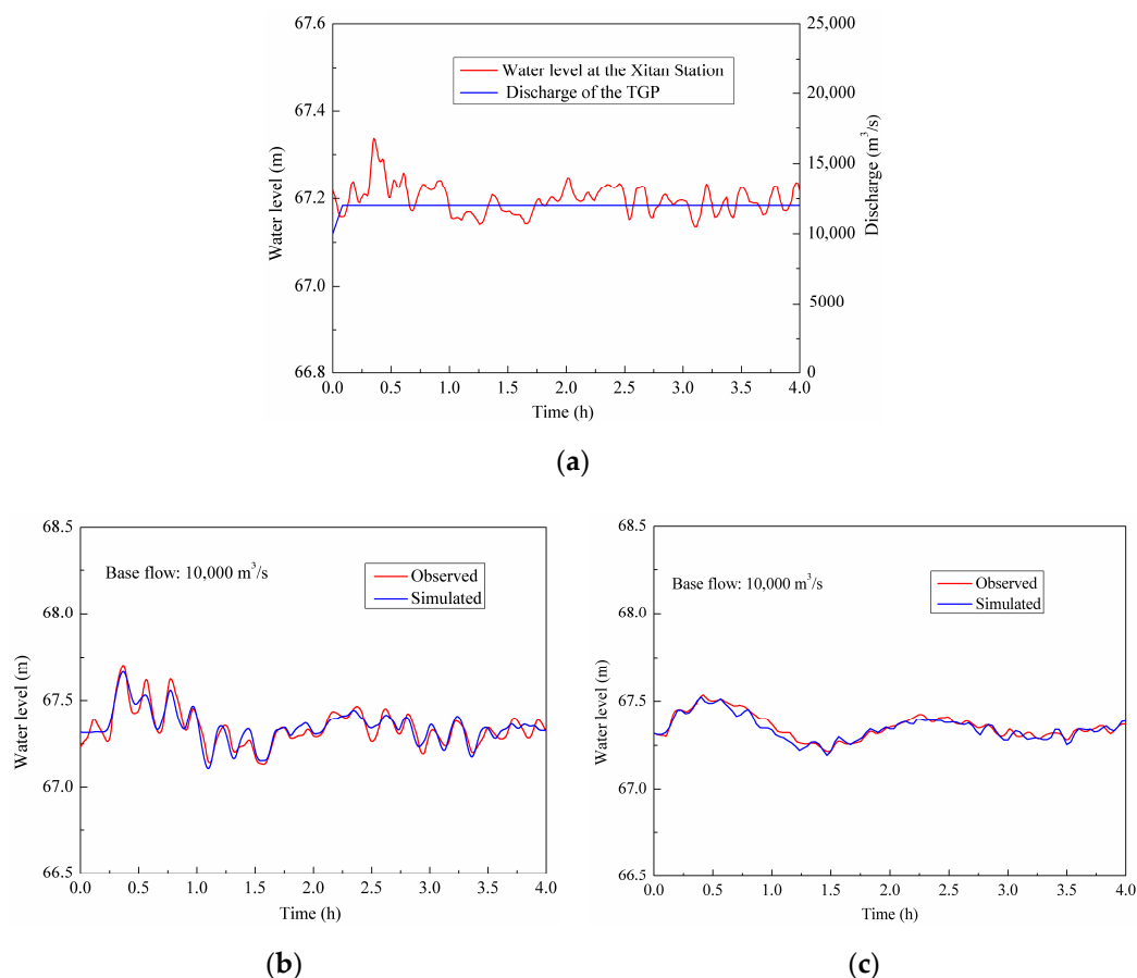
Figure 6. Boundary conditions and the simulated versus the measured water surface elevation. (a) Boundary conditions; (b) Water level at the lower lock head of the ship lift; (c) Water level at the entrance of the approach channel.
