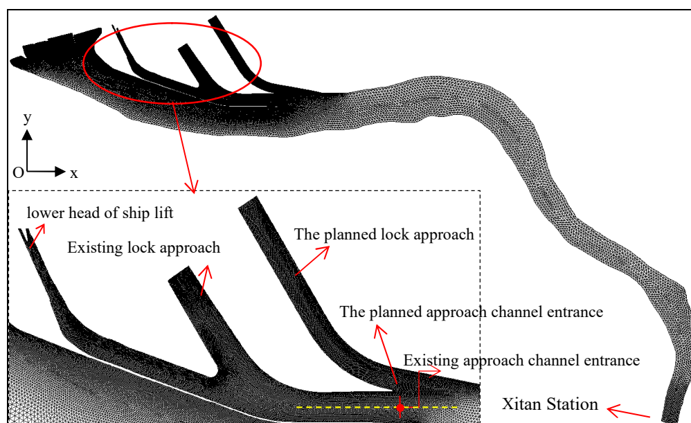
Figure 4. Computation domain and mesh generation.
