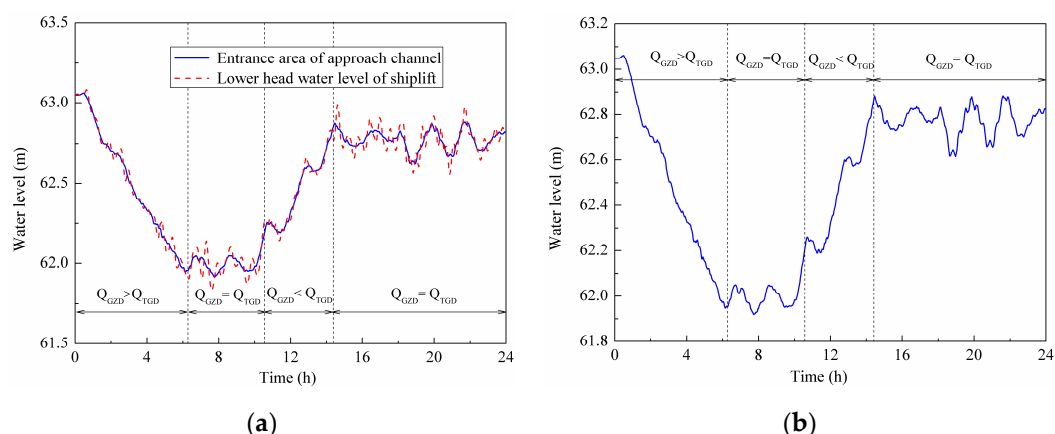
Figure 14. Water level variation process regarding single-peak regulation. (a) Approach channel entrance and lower lock head of the ship lift; (b) The planned approach channel entrance.
