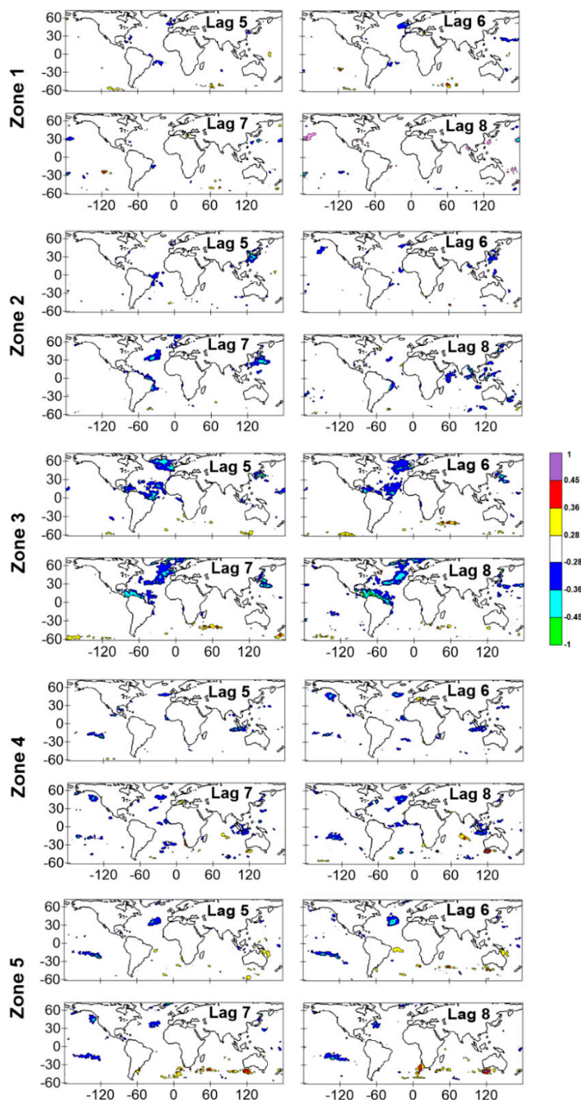
Figure 8. Maps showing the cross-correlations between April/May spring rainfall of each zone and SSTs for different oceanic regions at a lag time of 5–8 months.
