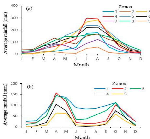
Figure 3. Mean monthly rainfall over Ethiopia for (a) nine summer zones (1951–2010) and (b) five spring zones (1951–2000).
