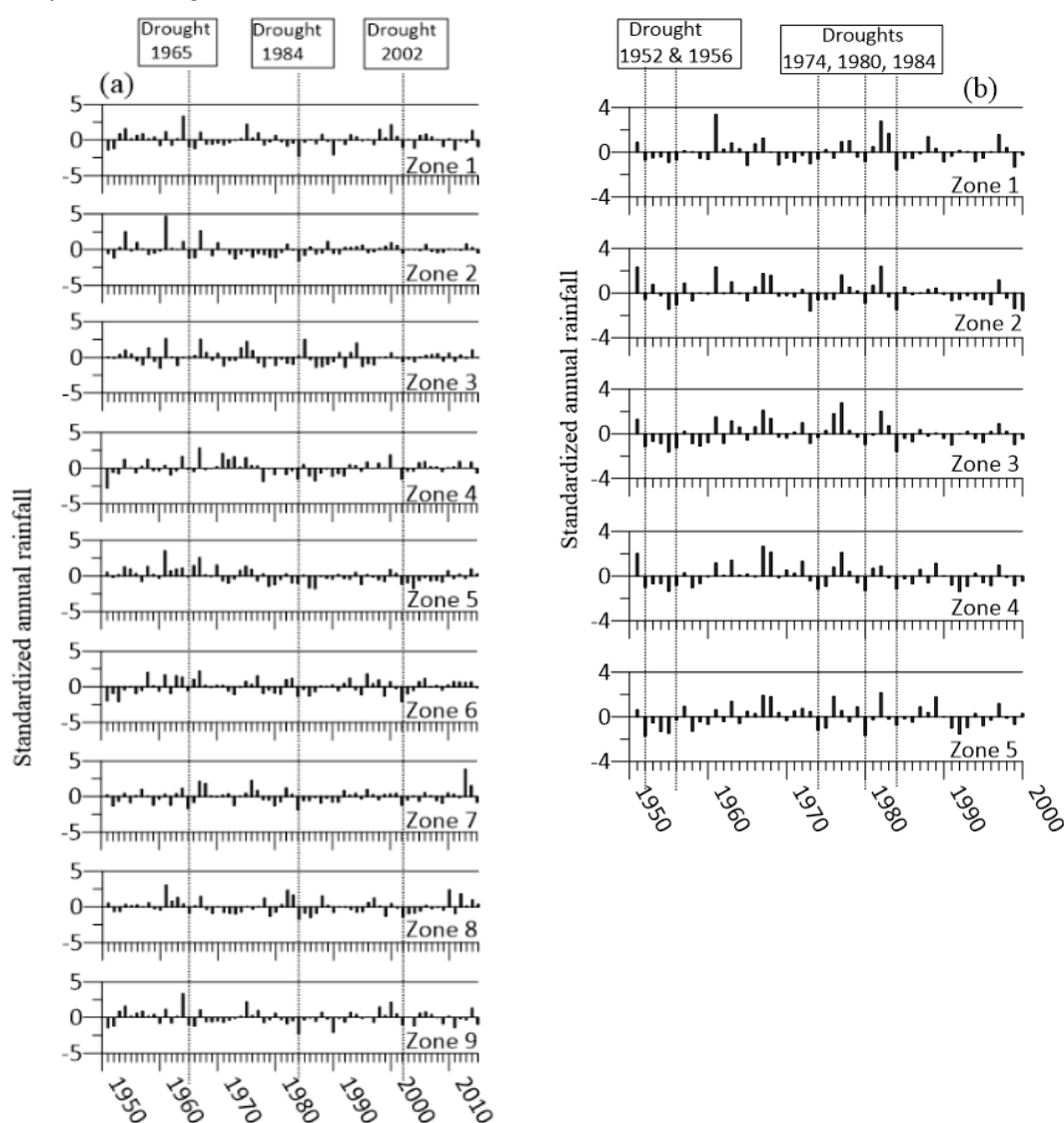
Figure 4. Standardized time-series plot of annual rainfall totals for (a) summer rainfall zones (1951–2015) and (b) spring rainfall zones (1951–2000).
