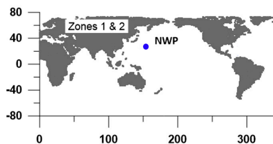
Figure 7. Extraction of common summer rainfall zones having the same significantly correlated SST regions ( r \geq 0.32 ) at the lag time of 7–8 months.
