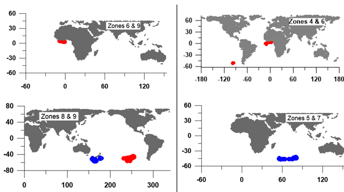
Figure 6. Extraction of common summer rainfall zones having the same significantly correlated SST regions ( r \geq 0.32 ) at lag times of 5–6 months ( left side ) and 6–7 months ( right side ). Red and blue colors indicate positive and negative correlations, respectively.
