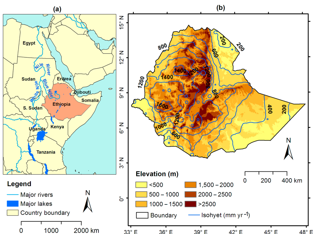
Figure 1. Location map of the study area: (a) Location of Ethiopia in eastern Africa; (b) A map of Ethiopia showing the mean annual rainfall distribution at 200 mm interval isohyets (blue lines) based on Climate Research Unit (CRU: https://www.cru.uea.ac.uk/data ) data of 1951–2015. The background provides elevation data extracted from a 90 m resolution Shuttle Radar Topographic Mission (SRTM: http://srtm.csi.cgiar.org/ ).
