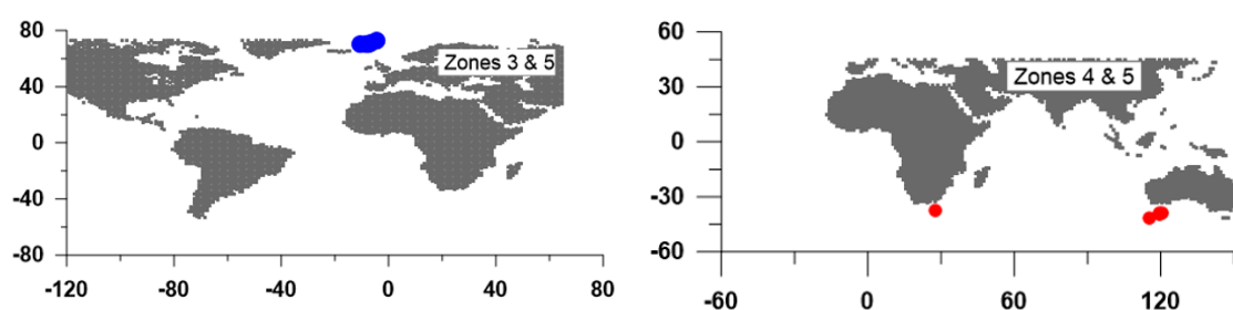
Figure 9. Extraction of common spring rainfall zones having the same significantly correlated SST regions ( r \geq 0.36 ) at a lag time of 6–7 months (left side) and 7–8 months (right side). Red and blue colors indicate positive and negative correlations, respectively.
