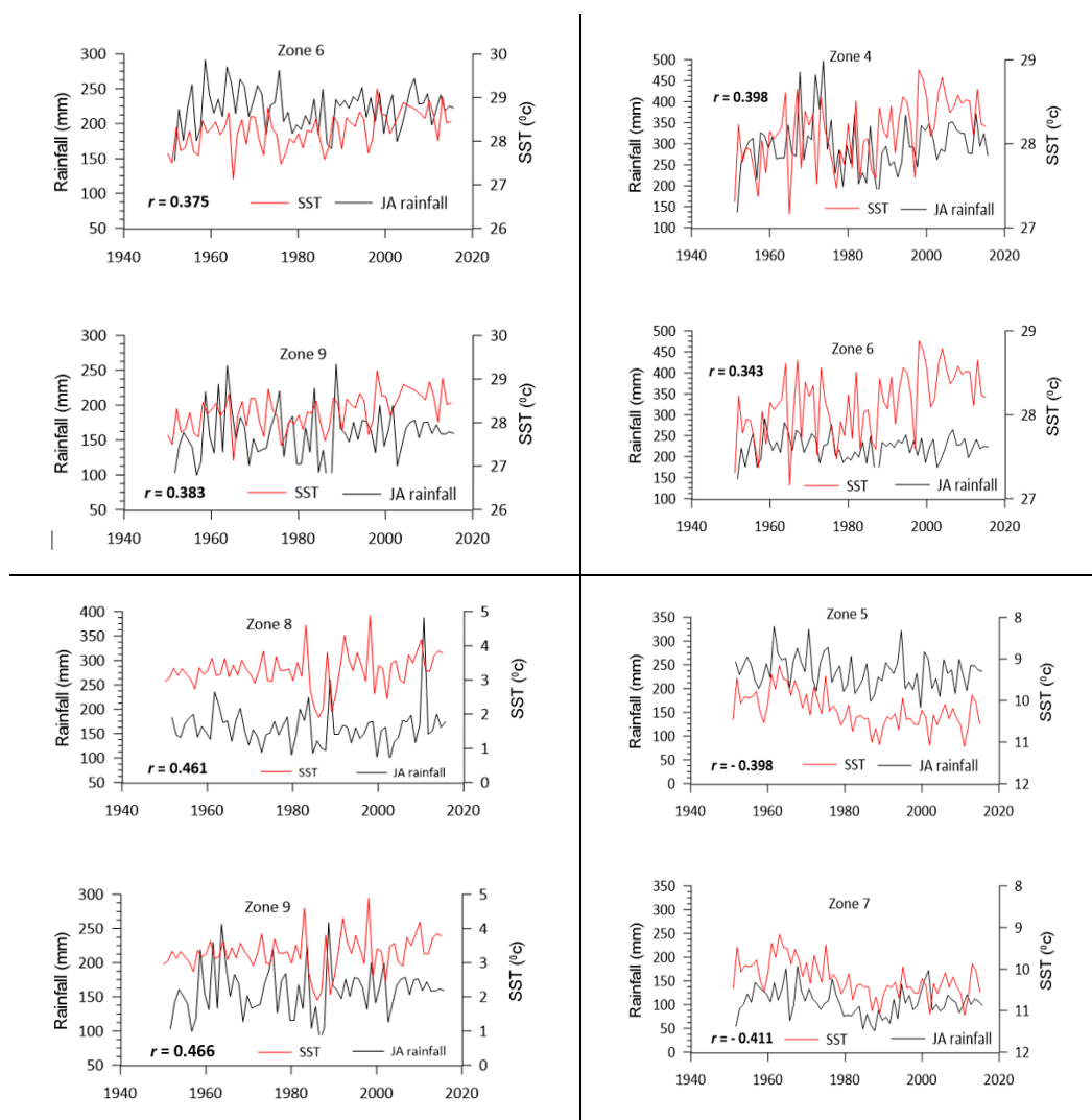
Figure 10. Significant cross-correlations between selected summer rainfall zones and oceanic SSTs at lag times of 5–6 months for zones (6 & 9) and (8 & 9) ( left side ) and 6–7 months for zones (4 & 6) and (5 & 7) ( right side ) for the rainfall time series (1951–2015). Zones 8 and 9 show the calculated ( r ) by subtracting positive and negative correlations.
