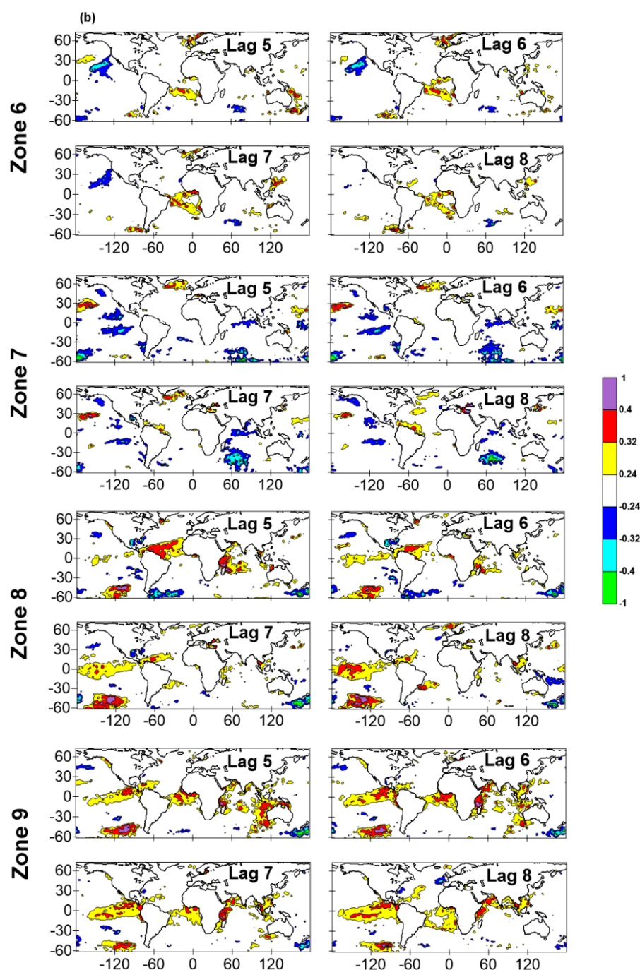
Figure 5. Maps (a) and (b) showing the nine summer rainfall zones with cross-correlations between July/August summer rainfall of each zone and sea surface temperatures (SSTs) for different oceanic regions at lag times of 5–8 months.
