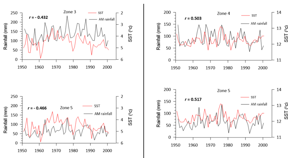
Figure 11. Significant cross-correlations between selected spring rainfall zones and oceanic SSTs at lag times of 6–7 months for zones 3 & 5 ( left side ) and 7–8 months for zones 4 & 5 ( right side ) for the rainfall time series (1951–2000).
