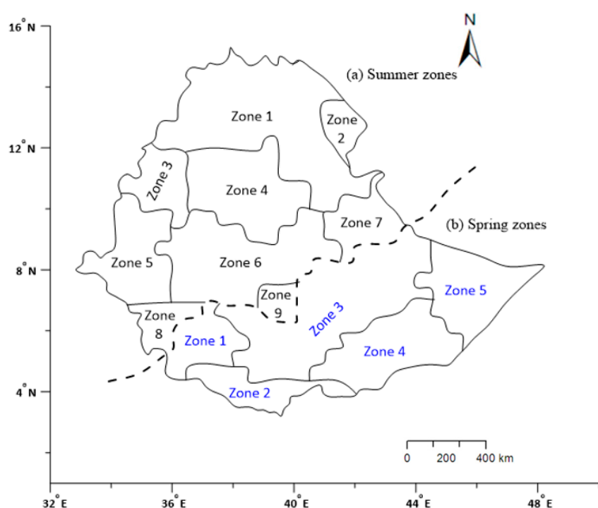
Figure 2. Homogenous rainfall zones over Ethiopia obtained from correlation analyses using monthly rainfall variability of summer rainfall peaks July–August (JA) and spring rainfall peaks April–May (AM).
