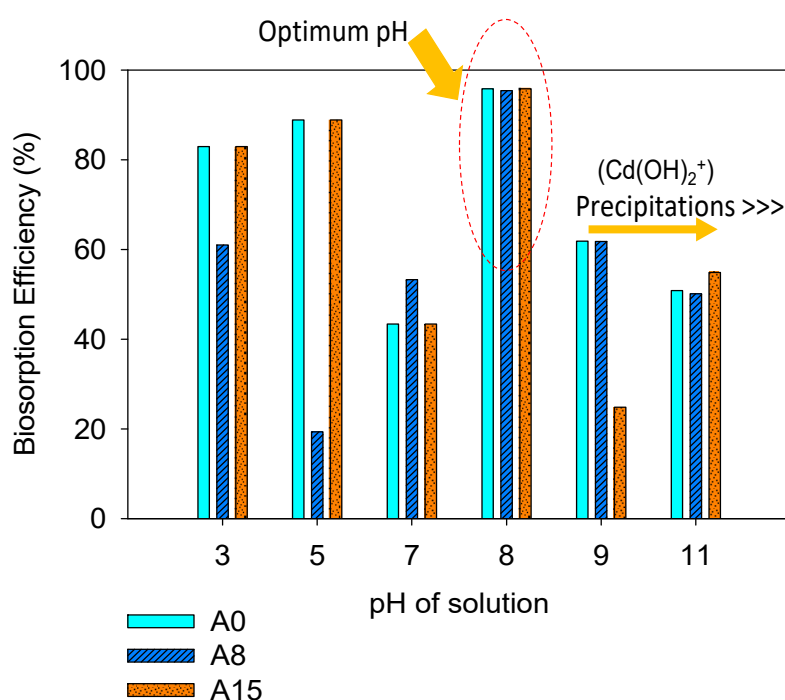
Figure 5. Effect of pH on sorption efficiency of \text{Cd}^{2+} onto dried biosorbent of Aphanothece sp. ( W_0 = 0.1 g/L, C_0 = 1 mg/L, t_{\text{contacts}} = 60 min, T = 30 °C, pH = 8).
