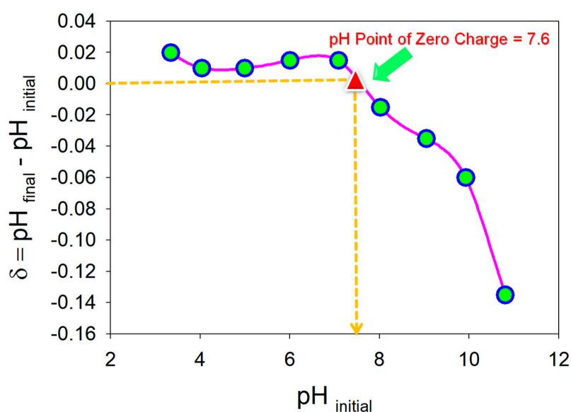
Figure 6. Point of zero charge plot ( \text{pH}_{\text{PZC}} ) of Aphanothece sp. ( W_0 = 0.1 g/L, C_0 = 1 mg/L, t_{\text{contacts}} = 60 min, T = 30 °C).
