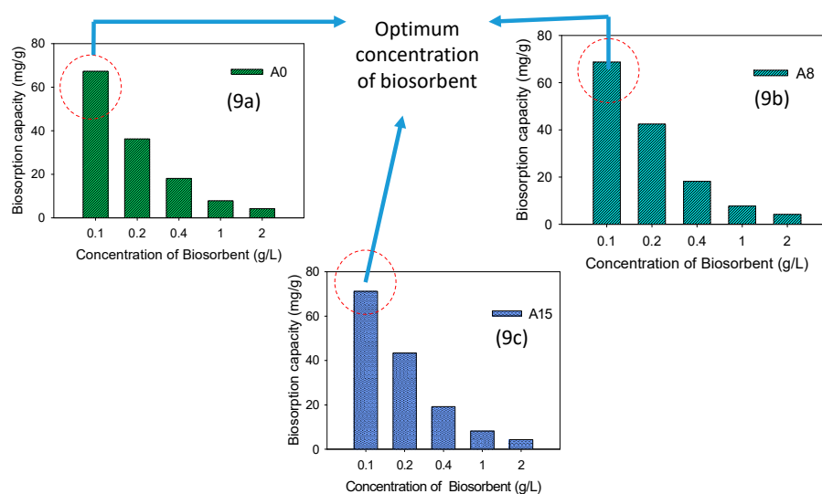
Figure 9. Effect of biosorbent concentration on sorption efficiency of \text{Cd}^{2+} onto dried biosorbent of Aphanotheca sp. for (a) adsorbent A0 ( \text{CO}_2 enrichment of 0.04%), (b) adsorbent A8 ( \text{CO}_2 enrichment of 8%) and (c) adsorbent A15 ( \text{CO}_2 enrichment of 15%) ( C_0 = 7.99 \text{ mg/L} , t_{\text{contacts}} = 60 \text{ min} , T = 30^\circ \text{C} ).
