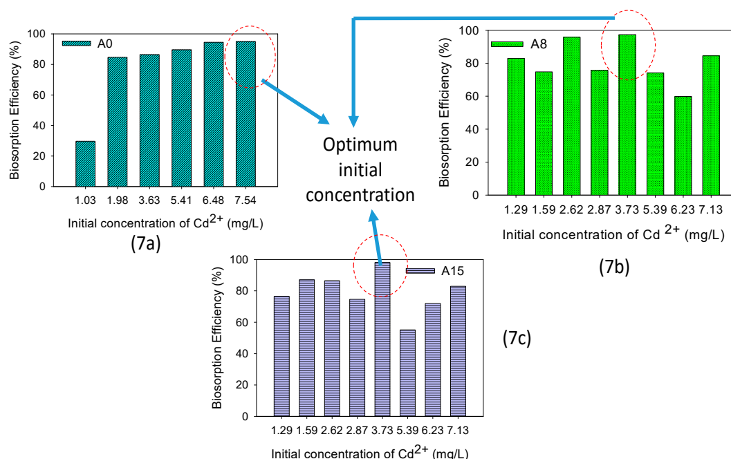
Figure 7. Effect of \text{Cd}^{2+} initial concentration on sorption efficiency of \text{Cd}^{2+} onto dried biosorbent of Aphanotheca sp. for (a) adsorbent A0 ( \text{CO}_2 enrichment of 0.04%), (b) adsorbent A8 ( \text{CO}_2 enrichment of 8%) and (c) adsorbent A15 ( \text{CO}_2 enrichment of 15%) ( W_0 = 0.1 g/L, t_{\text{contacts}} = 60 min, T = 30 °C).
