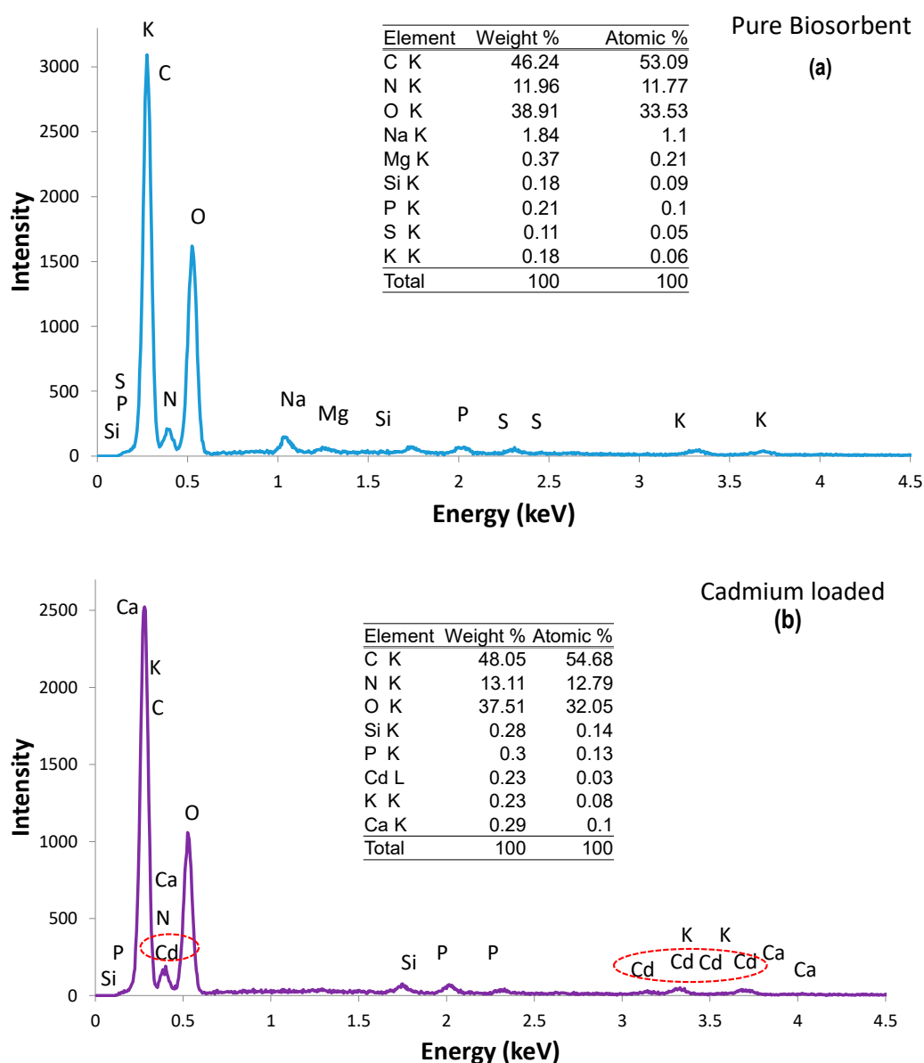
Figure 3. EDX spectra of dried biosorbent of Aphanothece sp. (a) before sorption and (b) after sorption using initial Cd concentration of 3 mg/L.
