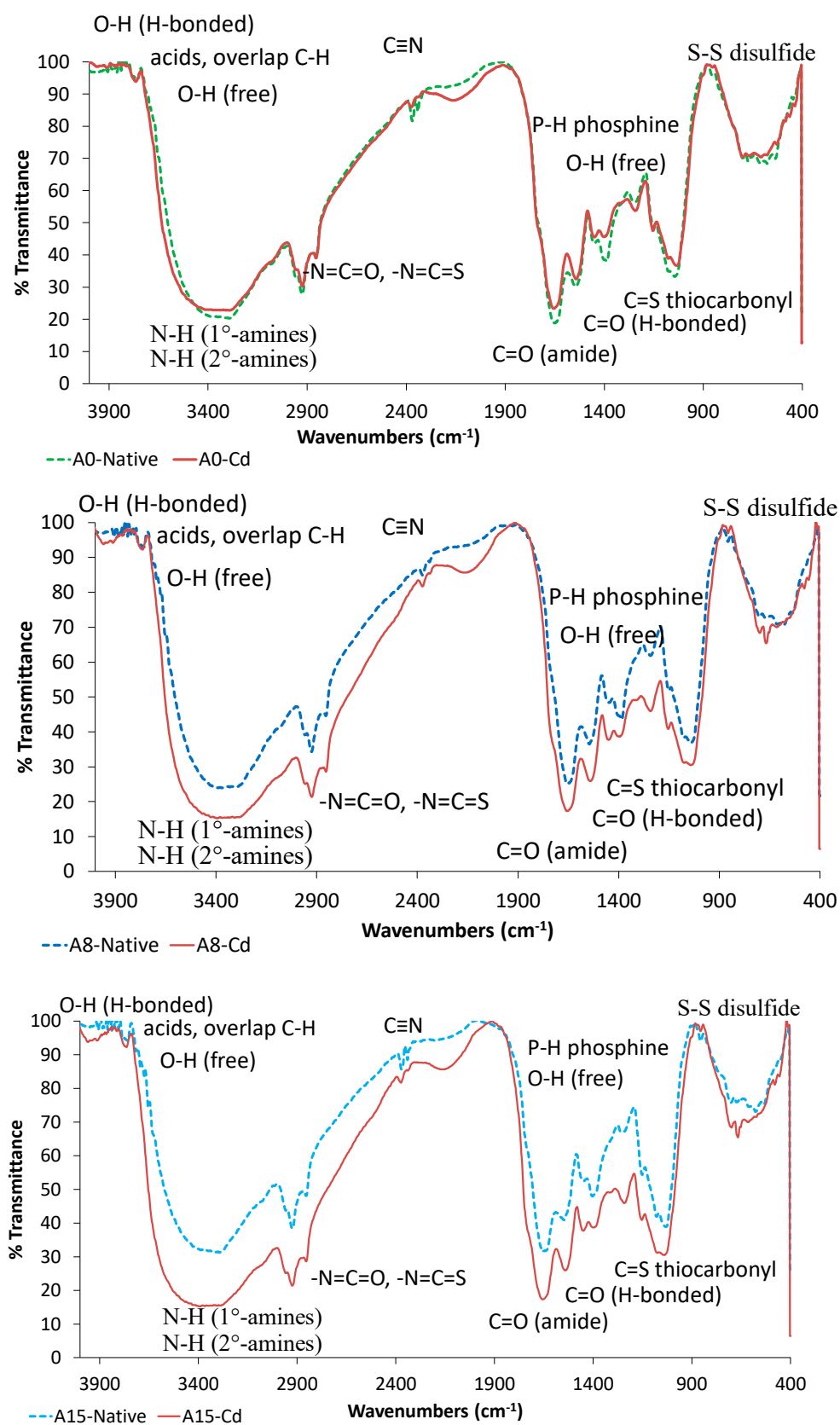
Figure 4. Spectra of dried biosorbent Aphanotheca sp. types A0, A8, and A15 before and after Cd 2+ sorption.
