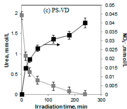
Figure 7. Behavior of urea and \text{NO}_3^- concentrations as a function of visible light irradiation time (after the dark period) obtained with FD LED dimming, S-VD LED dimming modulation, and PS-VD LED dimming modulation. Urea initial concentration: 250 mg/L in distilled water; solution volume: 250 mL; N-TiO 2 /PS amount: 120 g.
