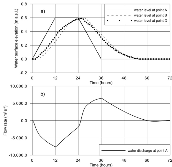
Figure 5. (a) Imposed boundary condition (point A–Baltiysk), and calculated (points B–Nowakowo and D–Kaliningrad) water levels and (b) calculated water discharge at point A in the Strait of Baltiysk.
